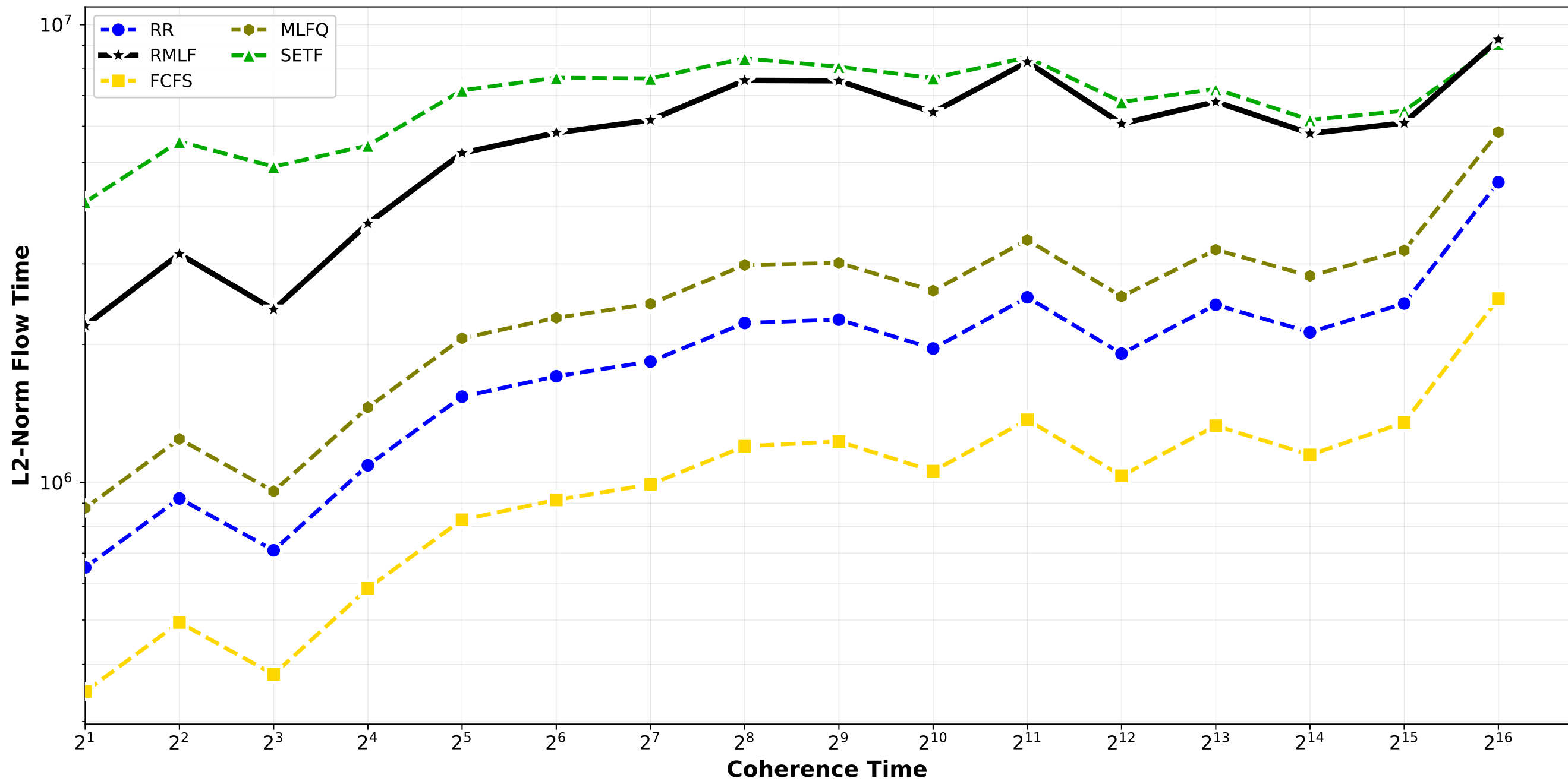
Non-Clairvoyant Algorithms - L2 Norm Flow Time normal_combination_random std6_std9 / pair_1
