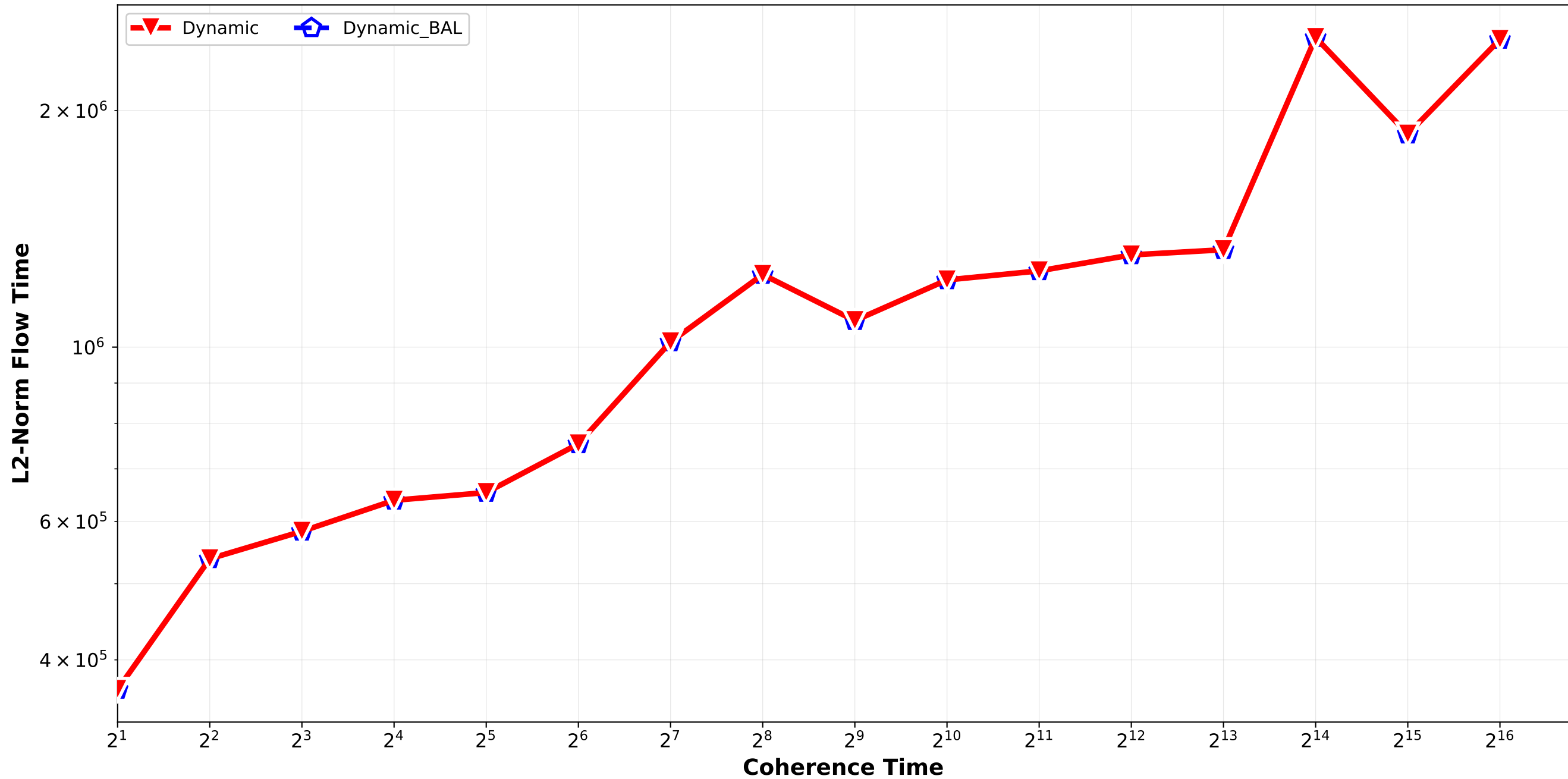
Dynamic vs Dynamic_BAL - L2 Norm Flow Time normal_combination_random std9_std12 / pair_2
