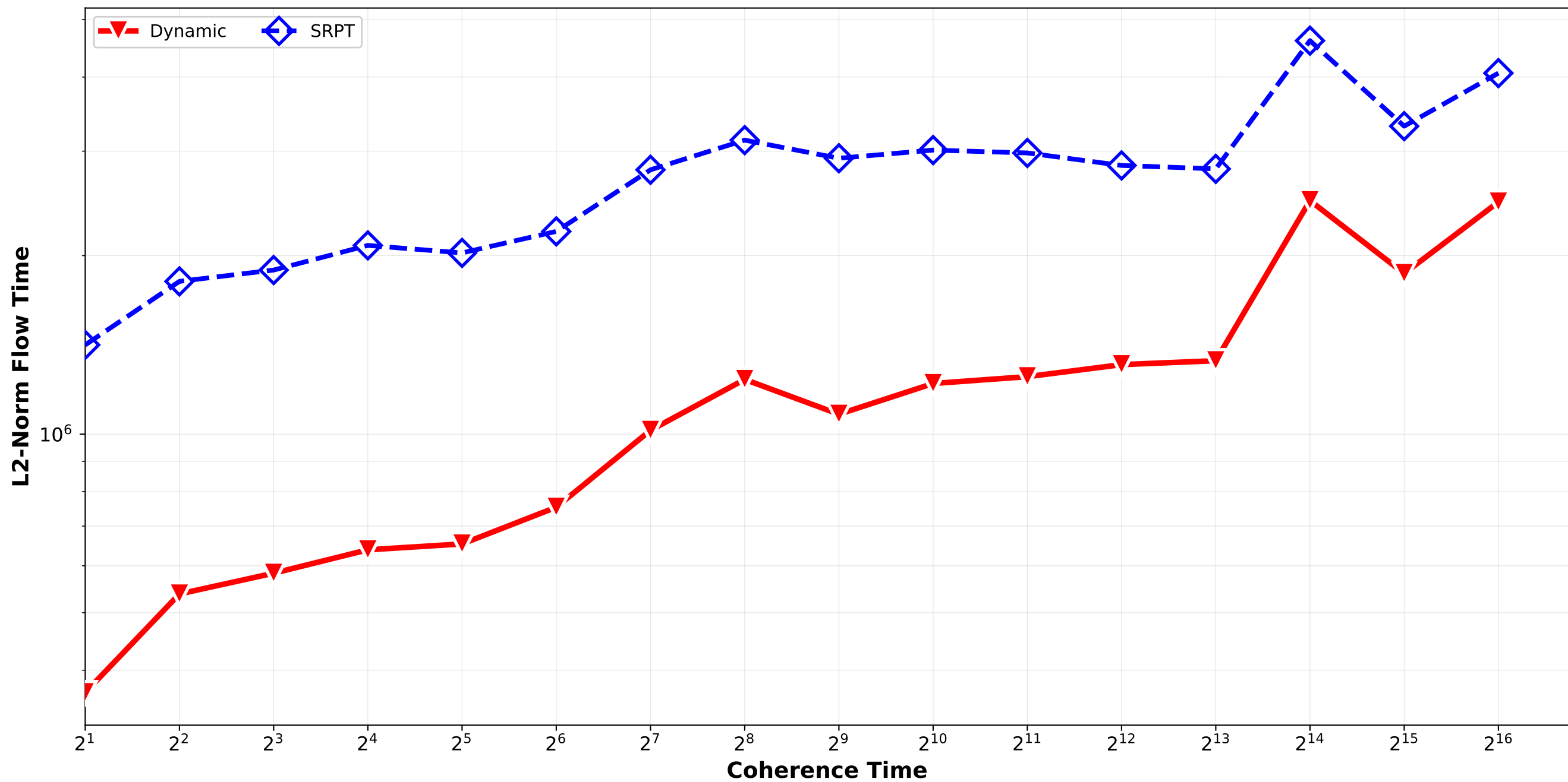
Dynamic vs SRPT - L2 Norm Flow Time normal_combination_random std9_std12 / pair_2
