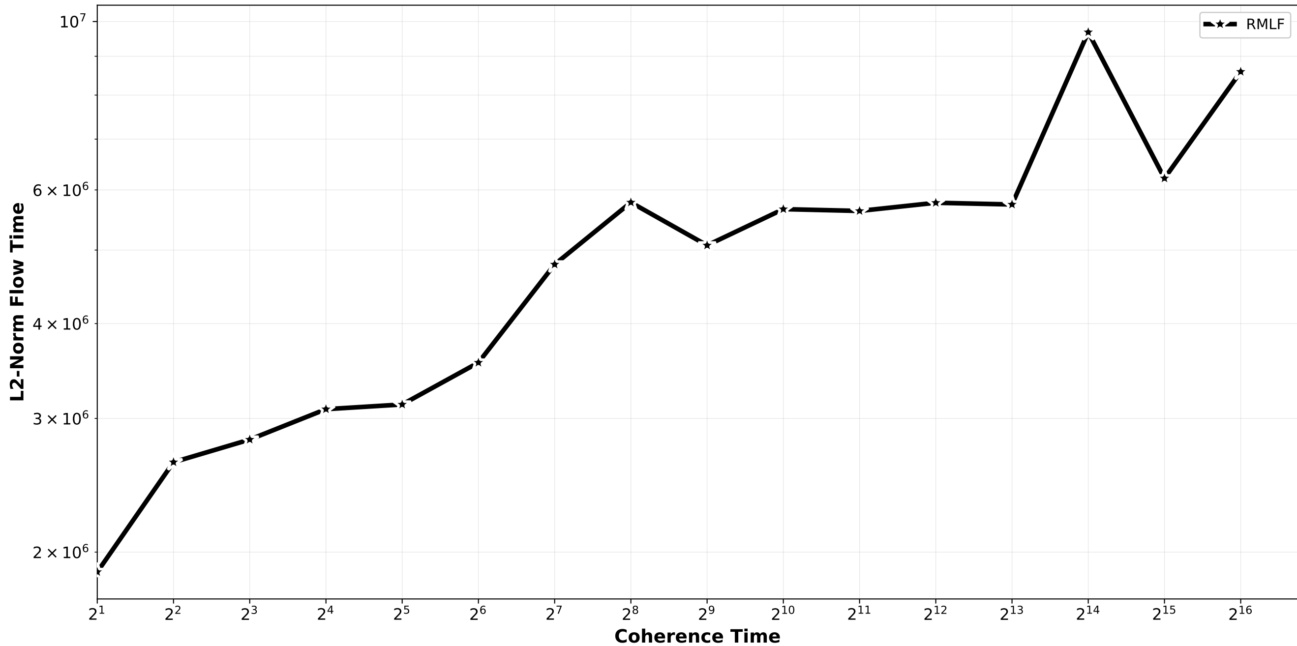
RFDynamic vs RMLF - L2 Norm Flow Time normal_combination_random std9_std12 / pair_2
