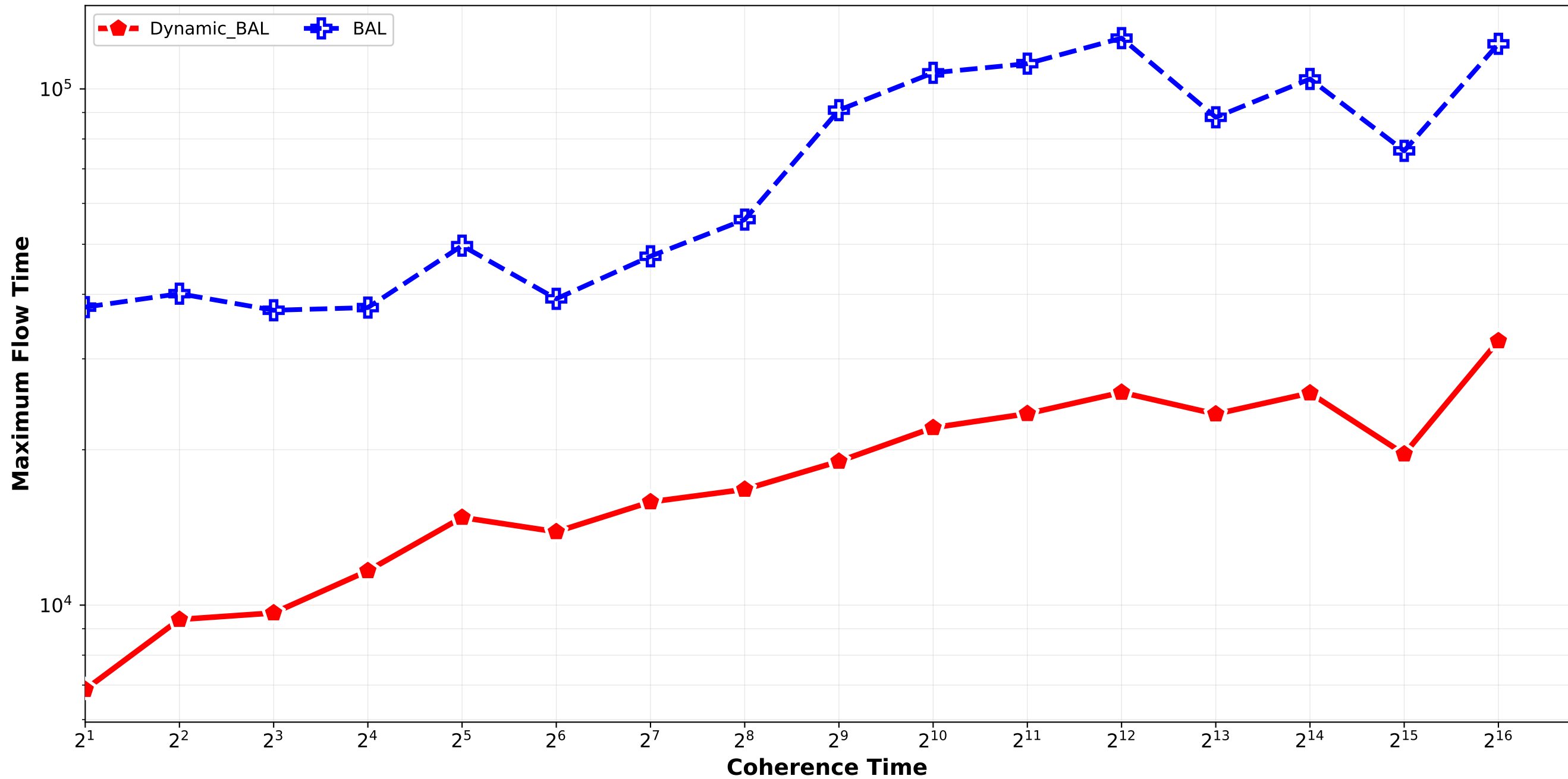
Dynamic_BAL vs BAL - Maximum Flow Time normal_combination_software std6_std9_std12_std15 / quadruplet_1
