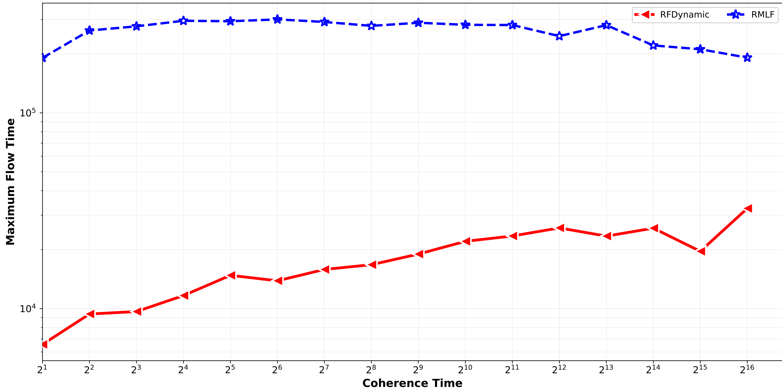
RFDynamic vs RMLF - Maximum Flow Time normal_combination_softrandom std6_std9_std12_std15 / quadruplet_1
