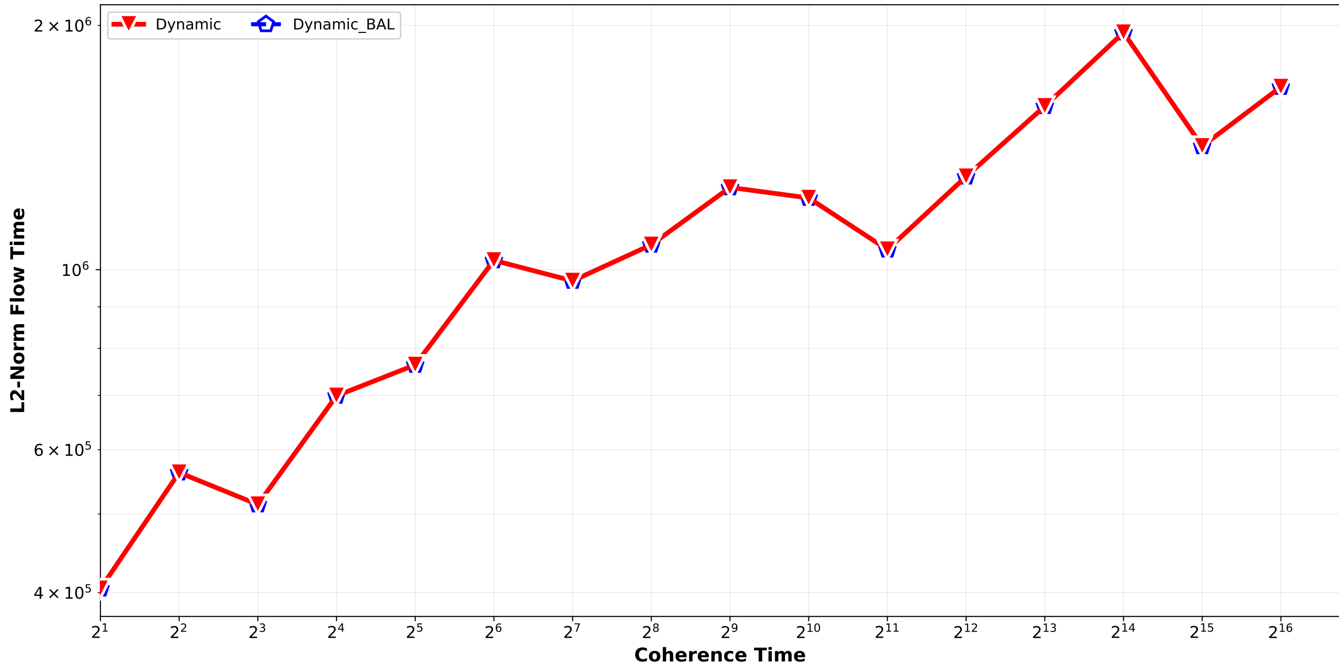
Dynamic vs Dynamic_BAL - L2 Norm Flow Time normal_combination_softrandom std9_std12_std15_std18 / quadruplet_2
