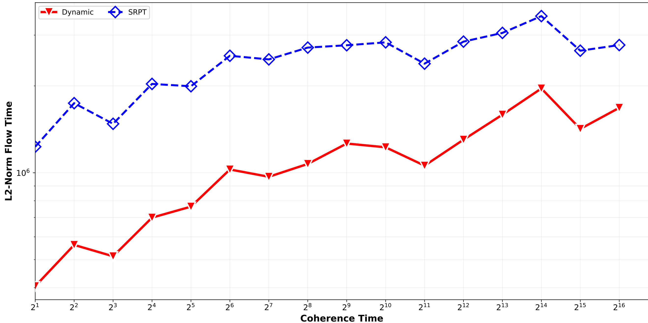
Dynamic vs SRPT - L2 Norm Flow Time normal_combination_softrandom std9_std12_std15_std18 / quadruplet_2
