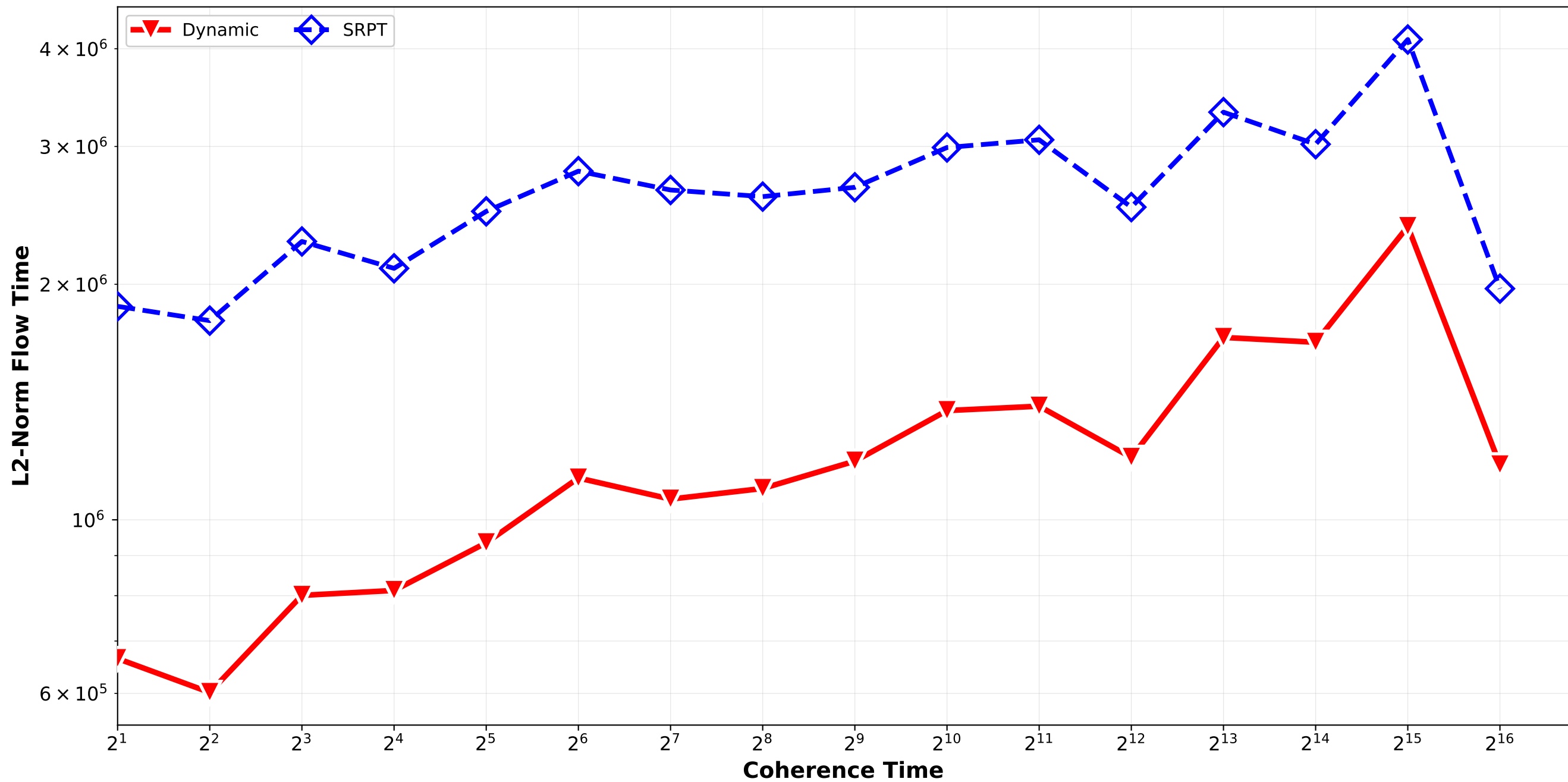
Dynamic vs SRPT - L2 Norm Flow Time normal_combination_softrandom std12_std15_std18 / triplet_3
