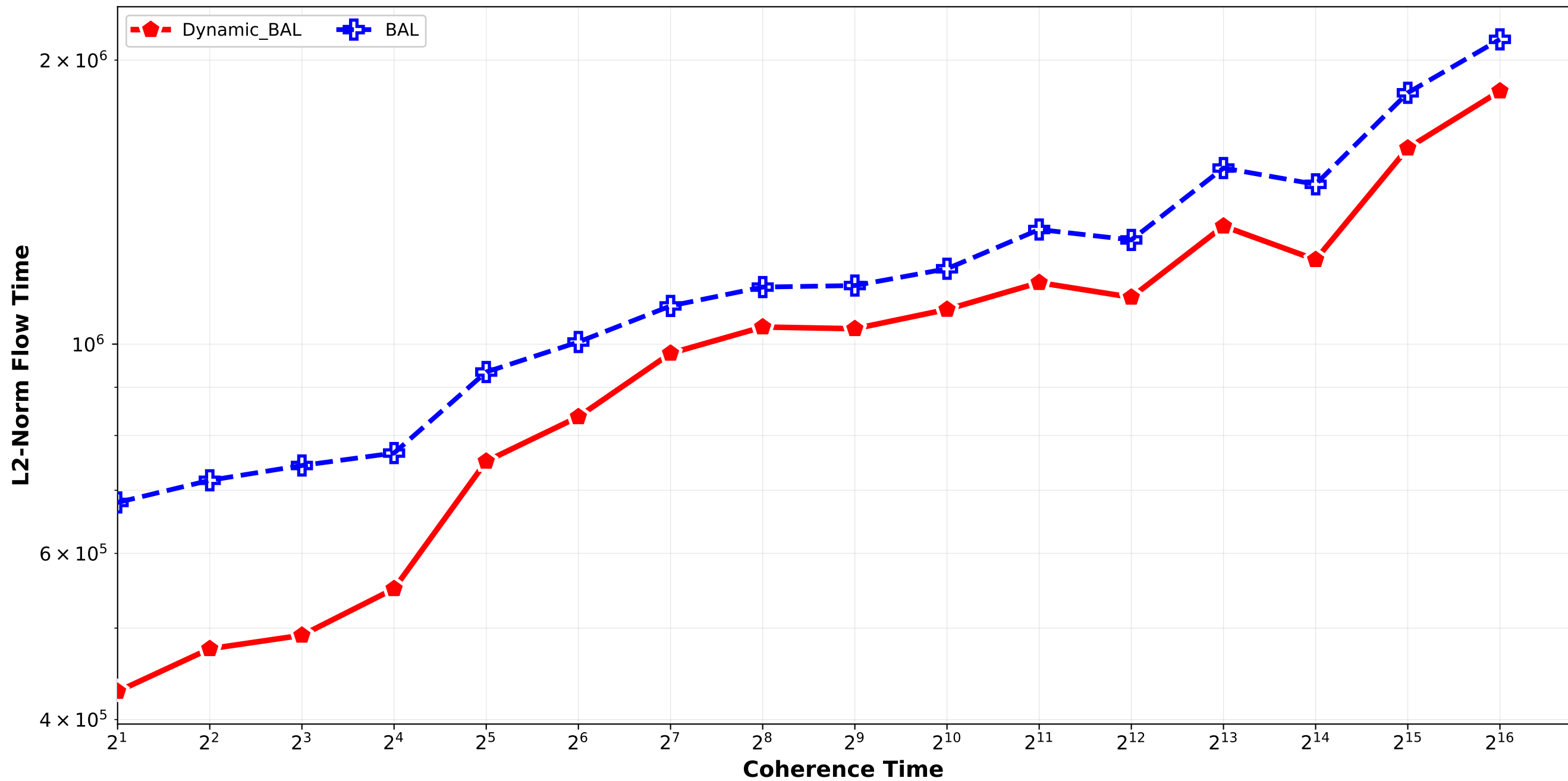
Dynamic_BAL vs BAL - L2 Norm Flow Time normal_combination_softrandom std6_std9_std12 / triplet_1
