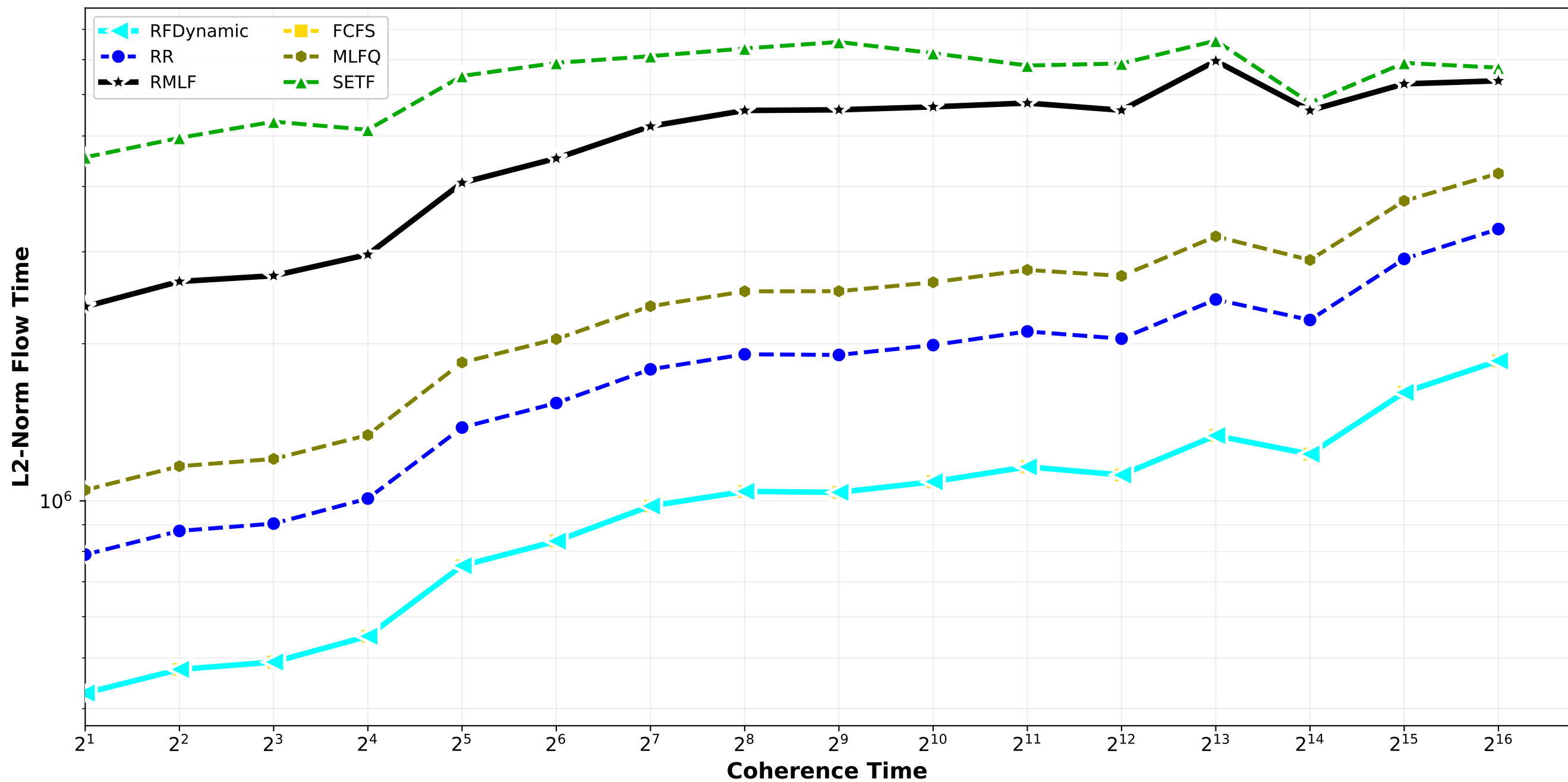
Non-Clairvoyant Algorithms - L2 Norm Flow Time normal_combination_softrandom std6_std9_std12 / triplet_1
