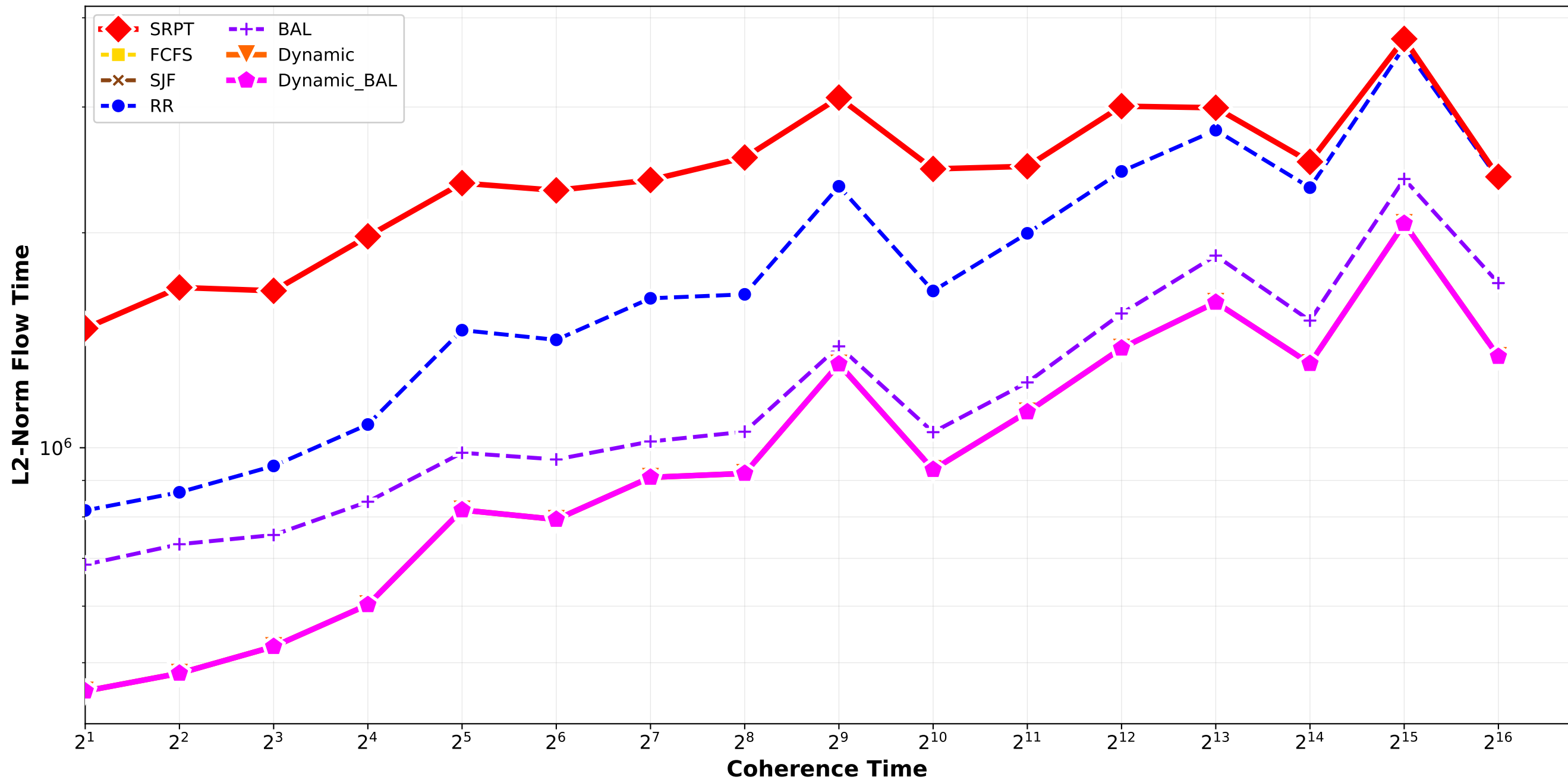
Clairvoyant Algorithms - L2 Norm Flow Time normal_combination_softrandom std9_std12_std15 / triplet_2
