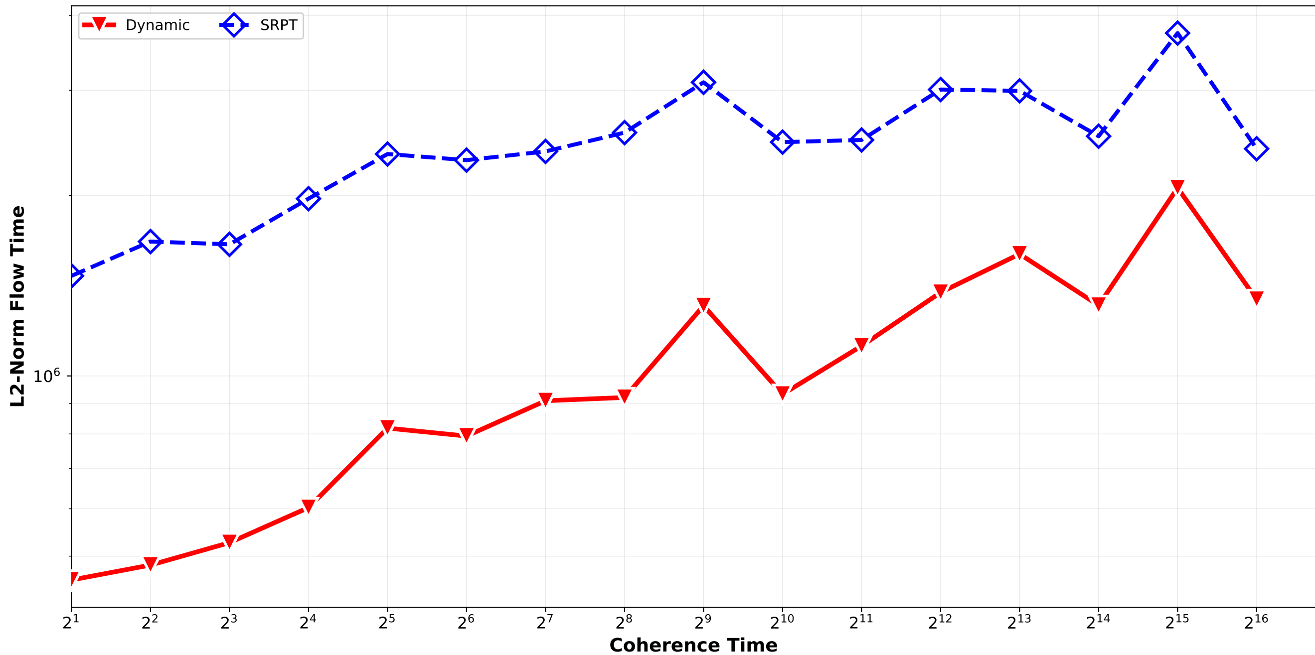
Dynamic vs SRPT - L2 Norm Flow Time normal_combination_softrandom std9_std12_std15 / triplet_2
