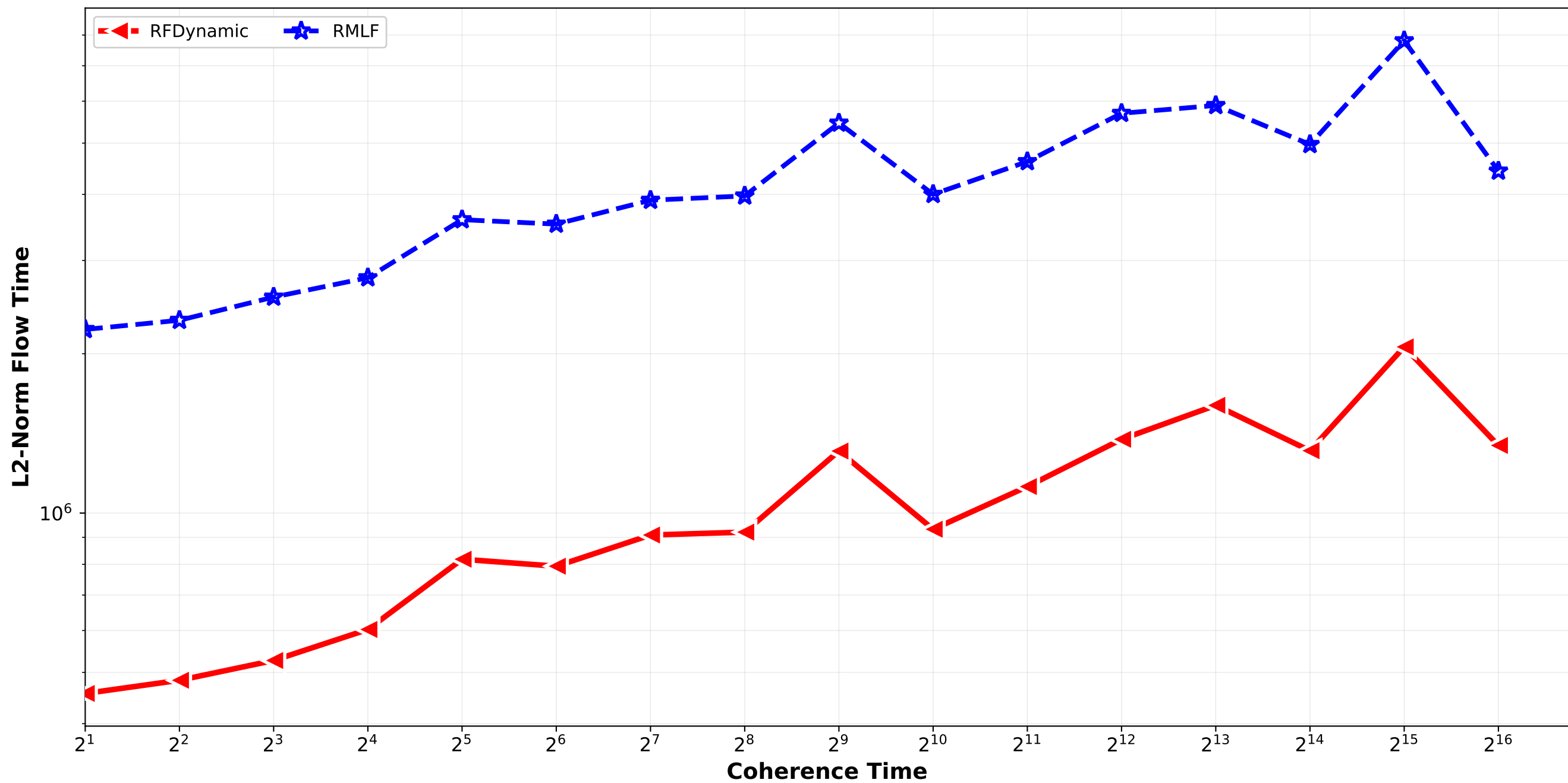
RFDynamic vs RMLF - L2 Norm Flow Time normal_combination_softmax std9_std12_std15 / triplet_2
