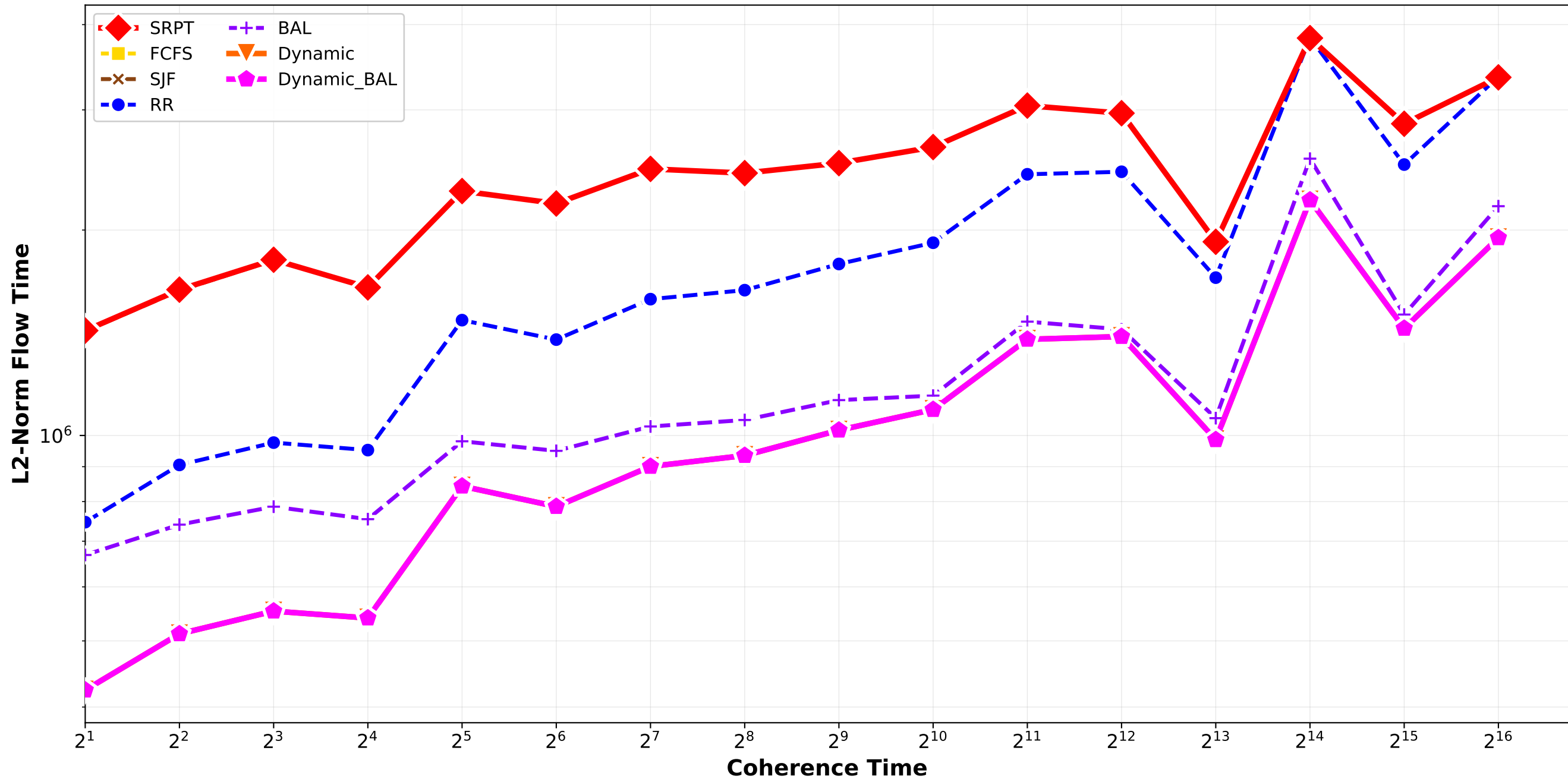
Clairvoyant Algorithms - L2 Norm Flow Time normal_combination_softrandom std12_std15 / pair_3
