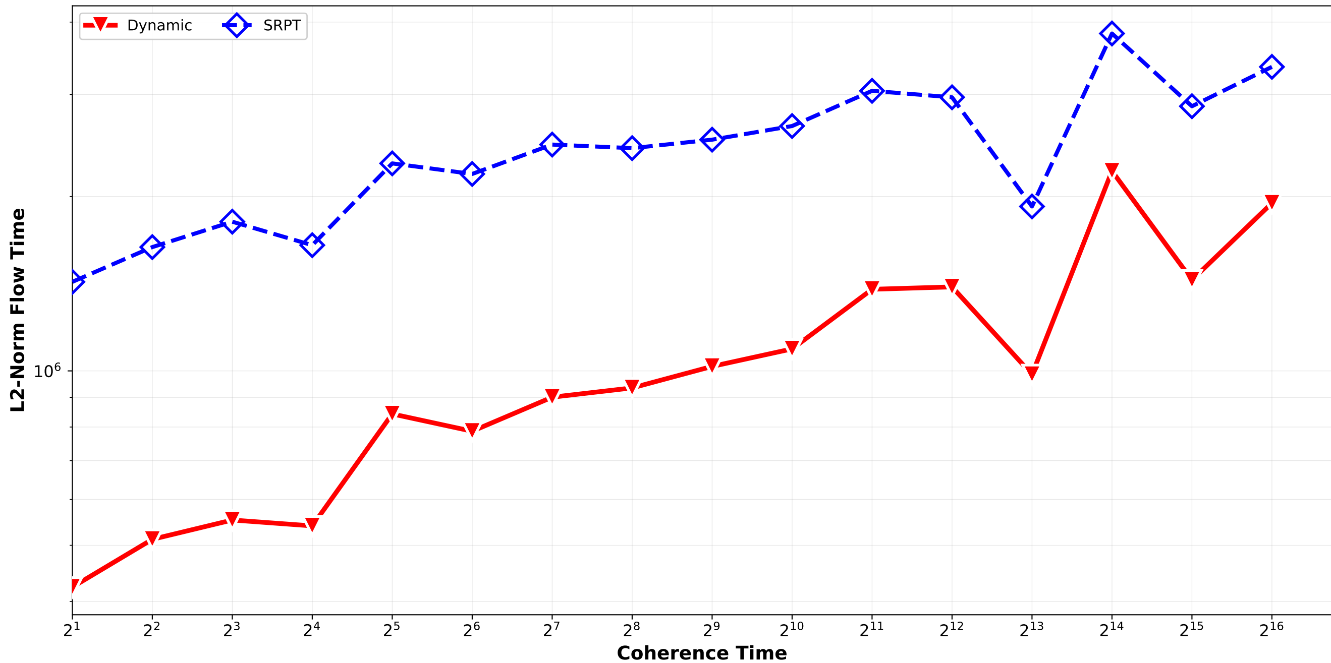
Dynamic vs SRPT - L2 Norm Flow Time normal_combination_softrandom std12_std15 / pair_3
