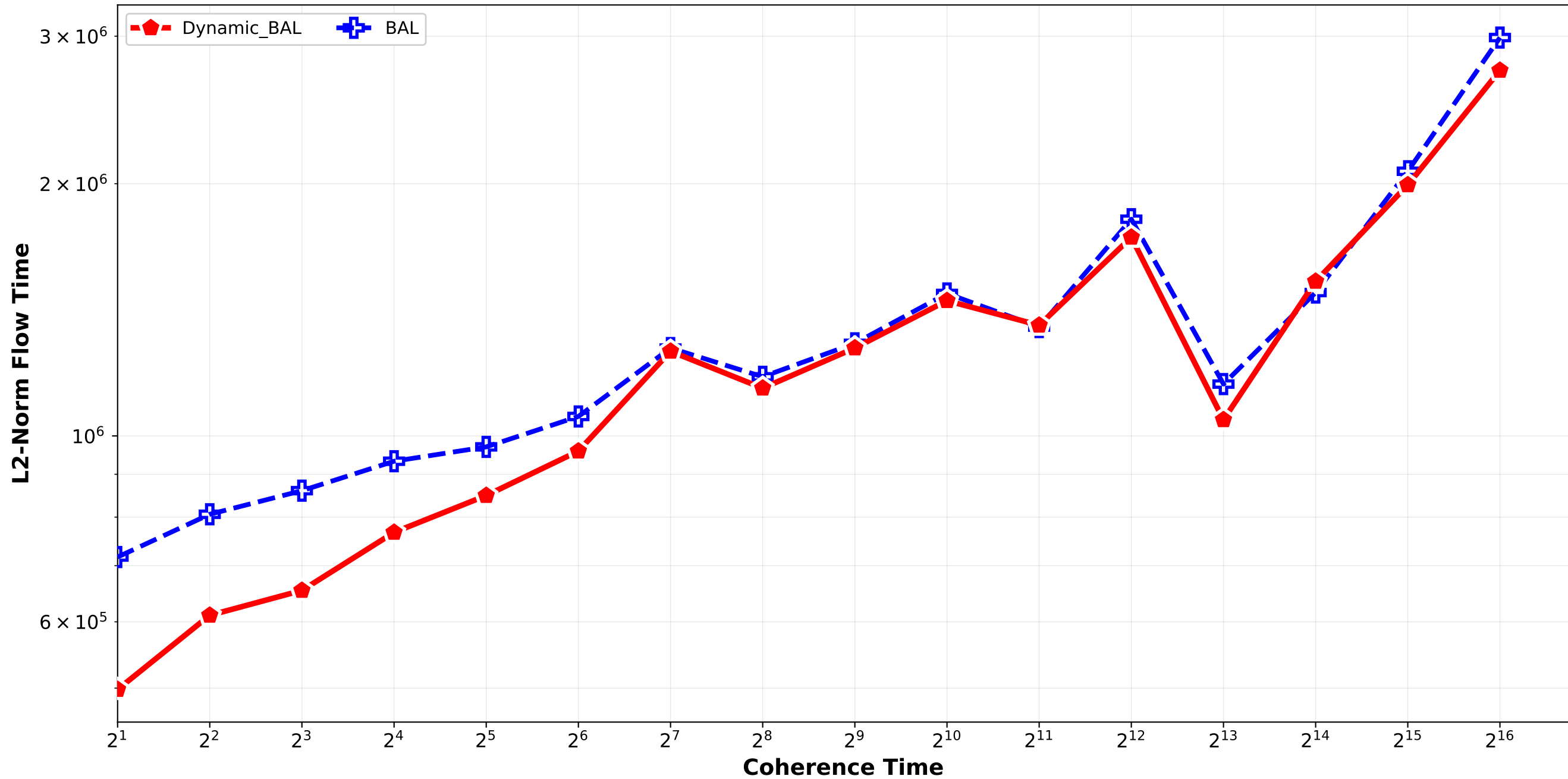
Dynamic_BAL vs BAL - L2 Norm Flow Time normal_combination_softrandom std15_std18 / pair_4
