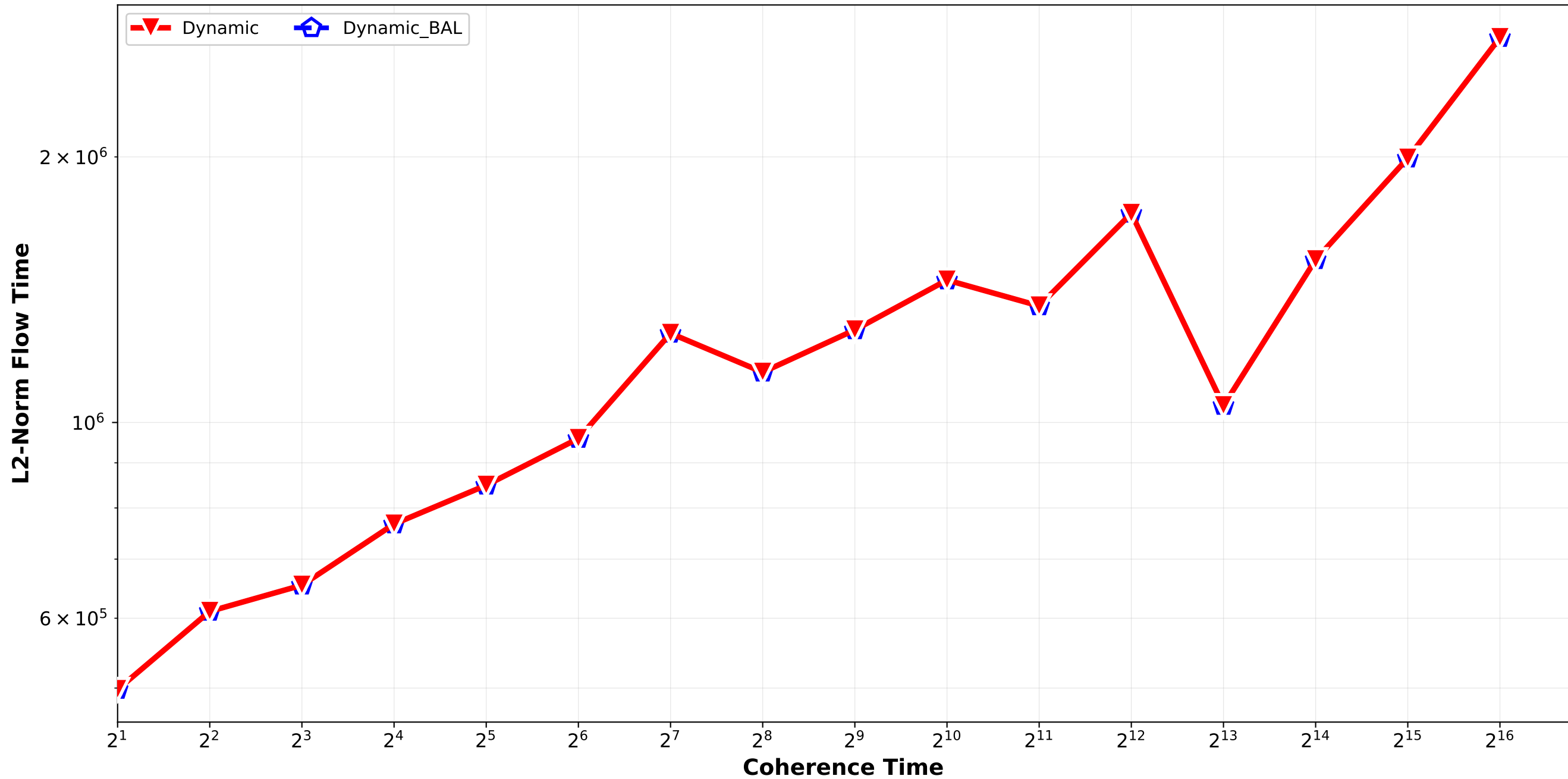
Dynamic vs Dynamic_BAL - L2 Norm Flow Time normal_combination_softrandom std15_std18 / pair_4
