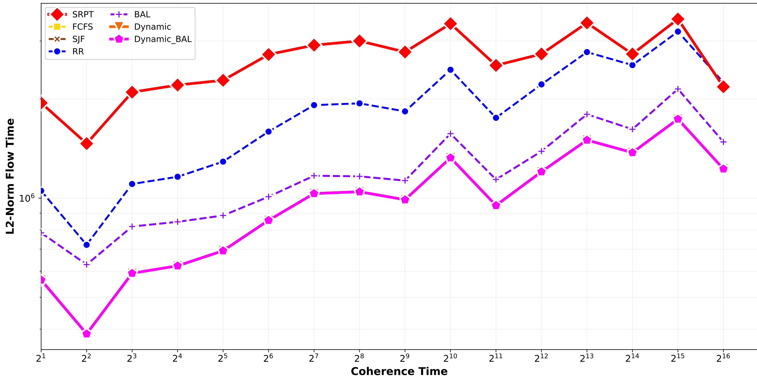
Clairvoyant Algorithms - L2 Norm Flow Time
