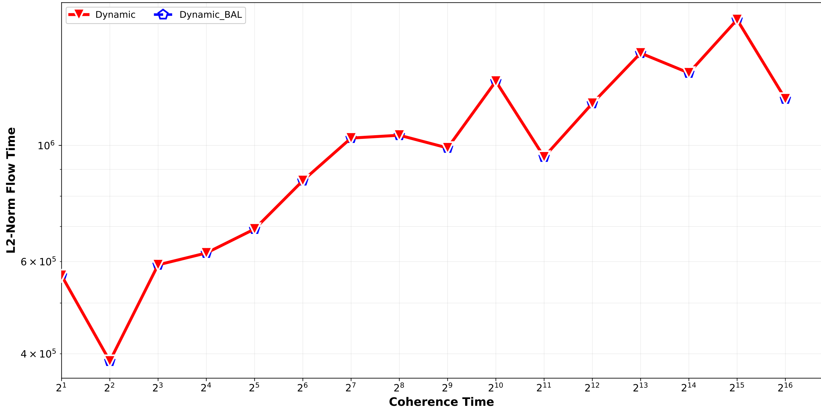
Dynamic vs Dynamic_BAL - L2 Norm Flow Time normal_combination_softrandom std6_std9 / pair_1
