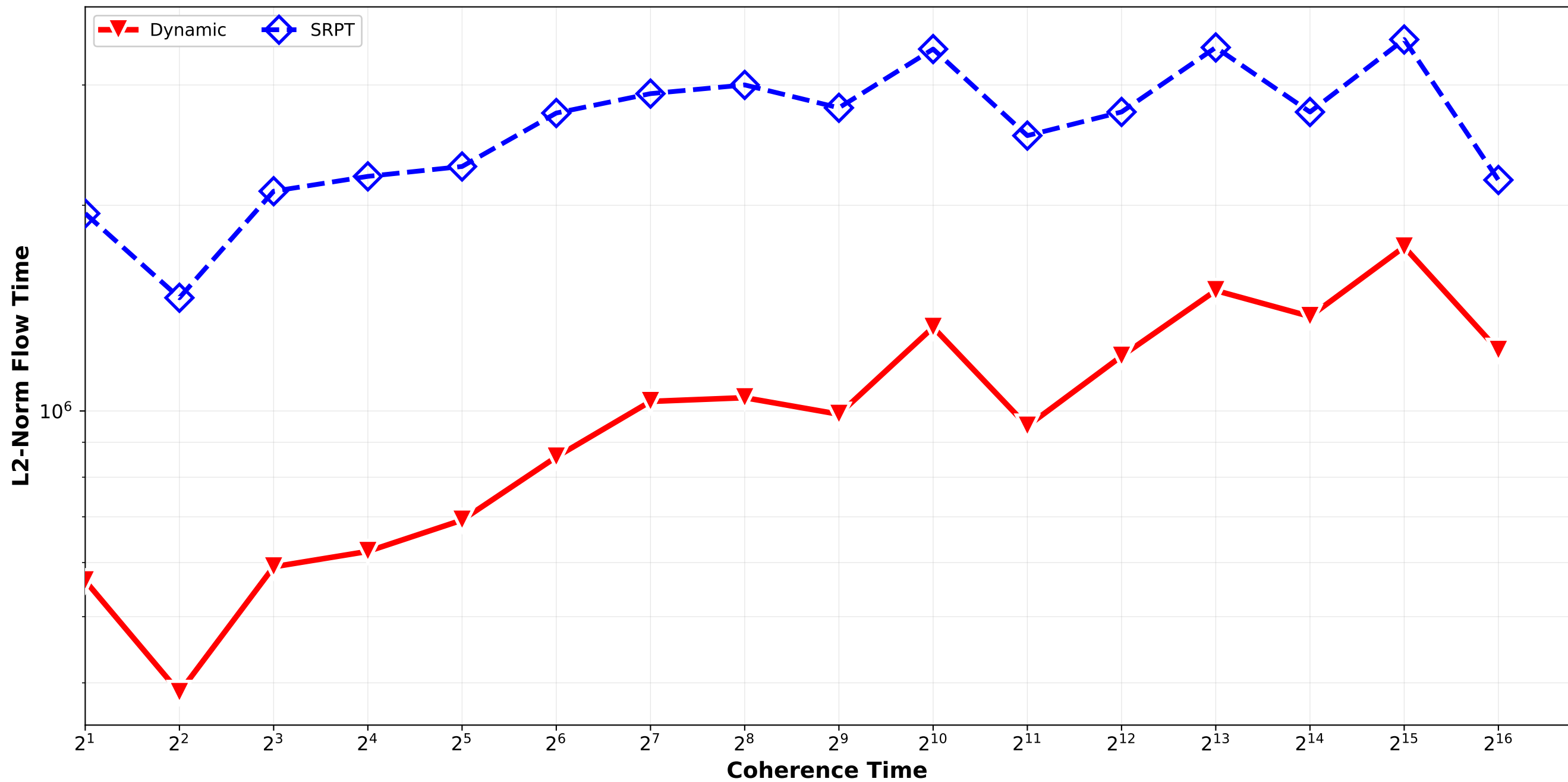
Dynamic vs SRPT - L2 Norm Flow Time normal_combination_softrandom std6_std9 / pair_1
