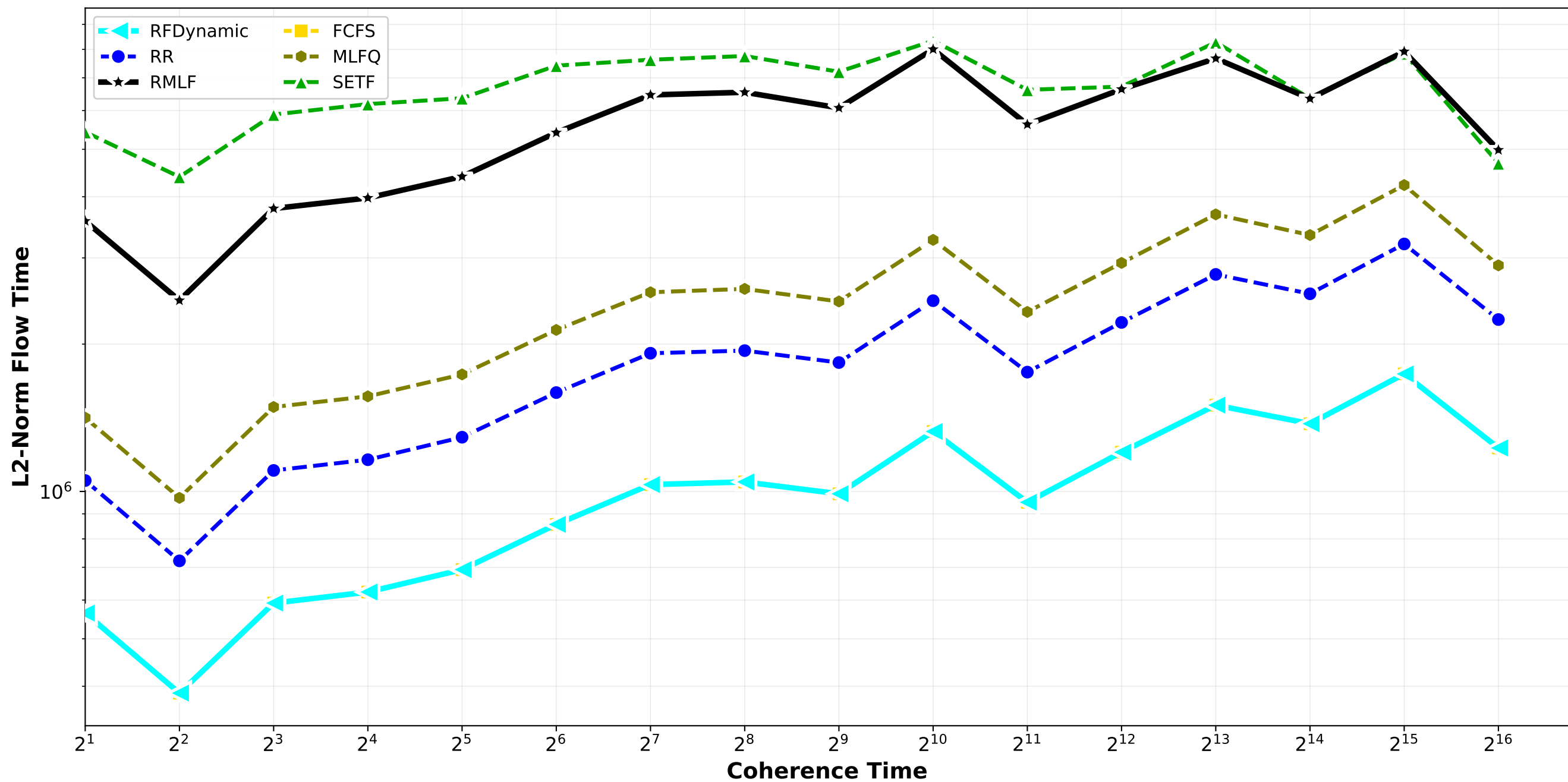
Non-Clairvoyant Algorithms - L2 Norm Flow Time normal_combination_softrandom std6_std9 / pair_1
