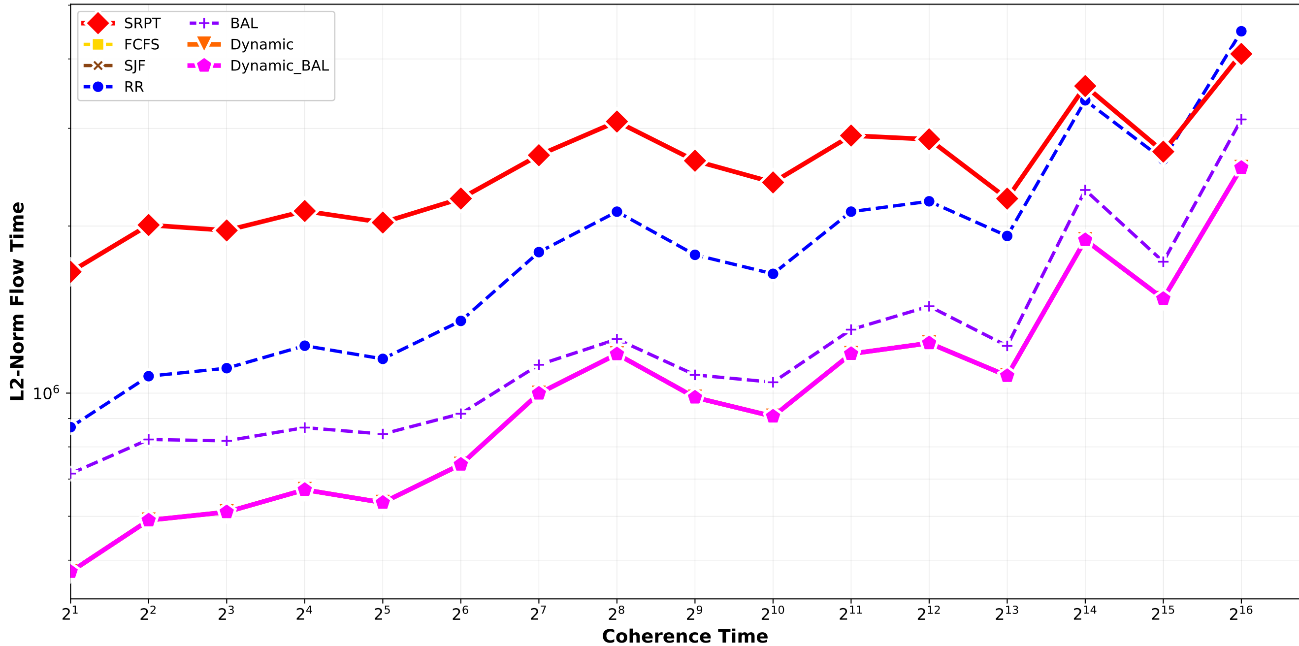
Clairvoyant Algorithms - L2 Norm Flow Time normal_combination_softrandom std9_std12 / pair_2
