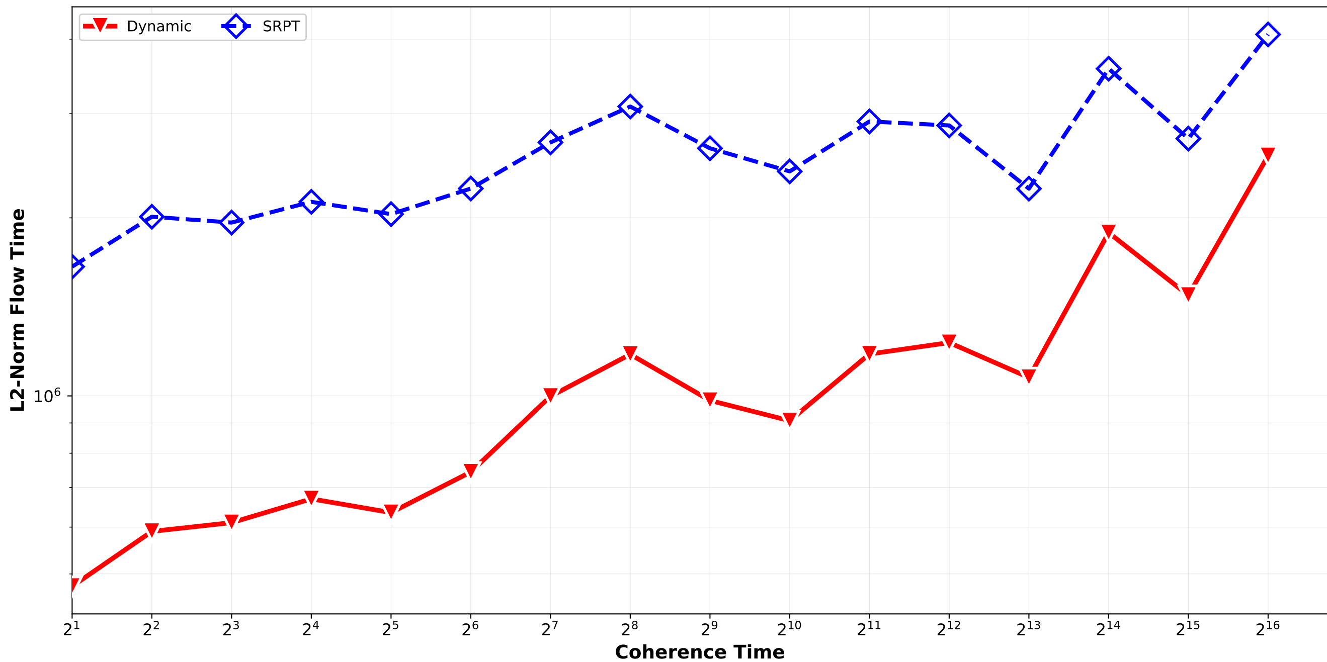
Dynamic vs SRPT - L2 Norm Flow Time normal_combination_softrandom std9_std12 / pair_2
