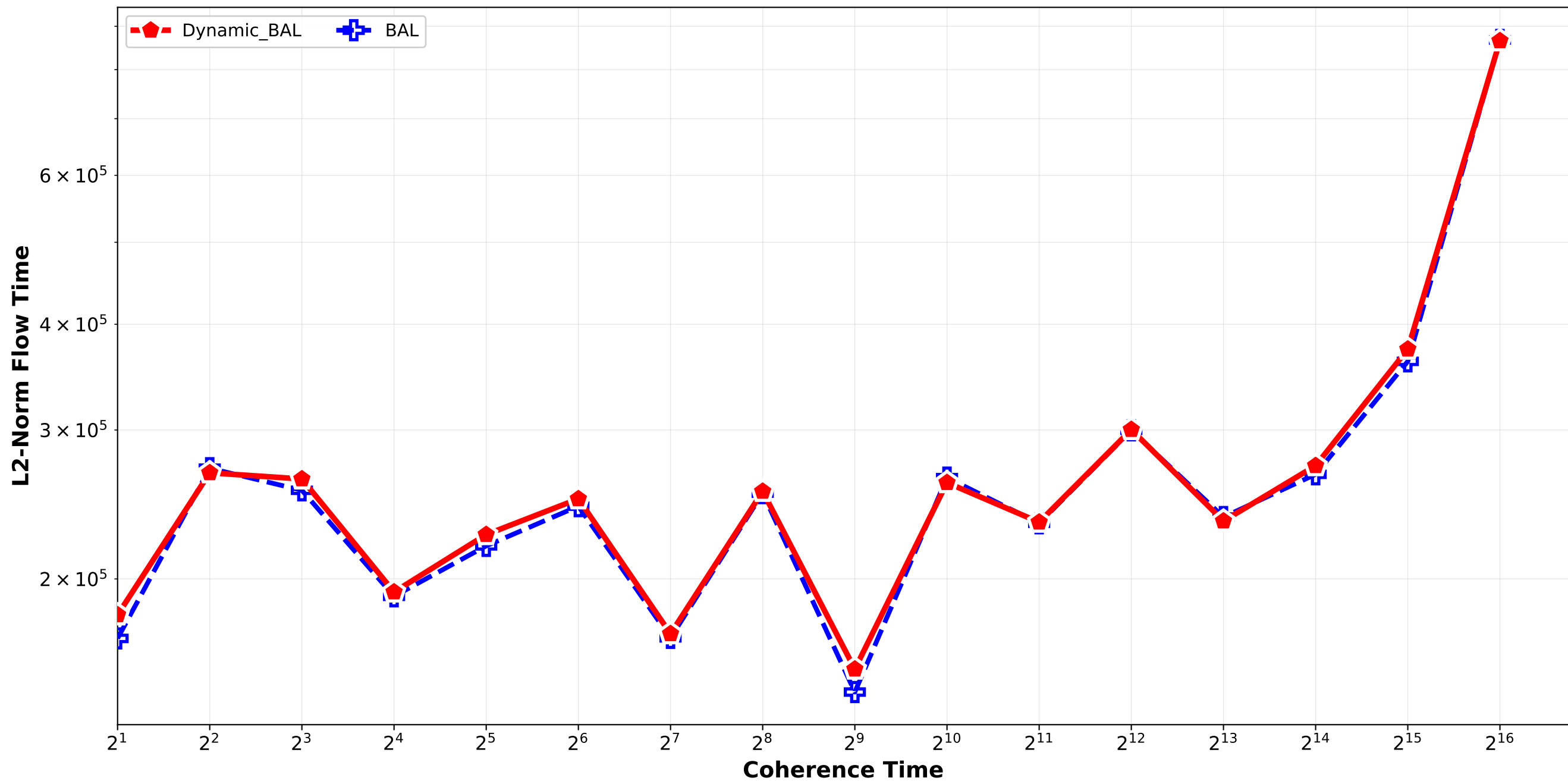
Dynamic_BAL vs BAL - L2 Norm Flow Time Bounded_Pareto_combination_random H512_H4096_H32768_H262144 / quadruplet_2
