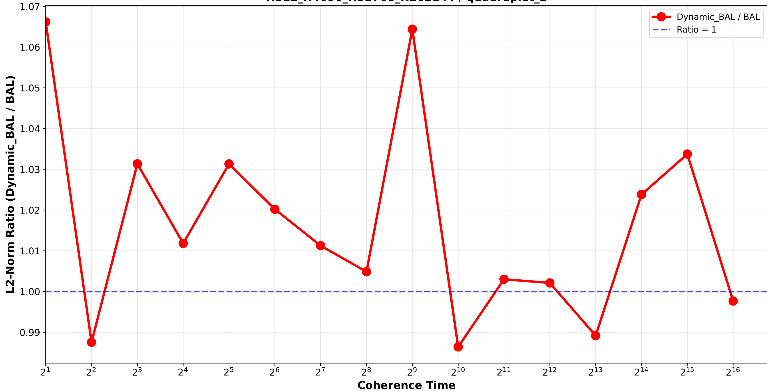
Dynamic_BAL vs BAL - L2 Norm Ratio Bounded_Pareto_combination_random H512_H4096_H32768_H262144 / quadruplet_2
