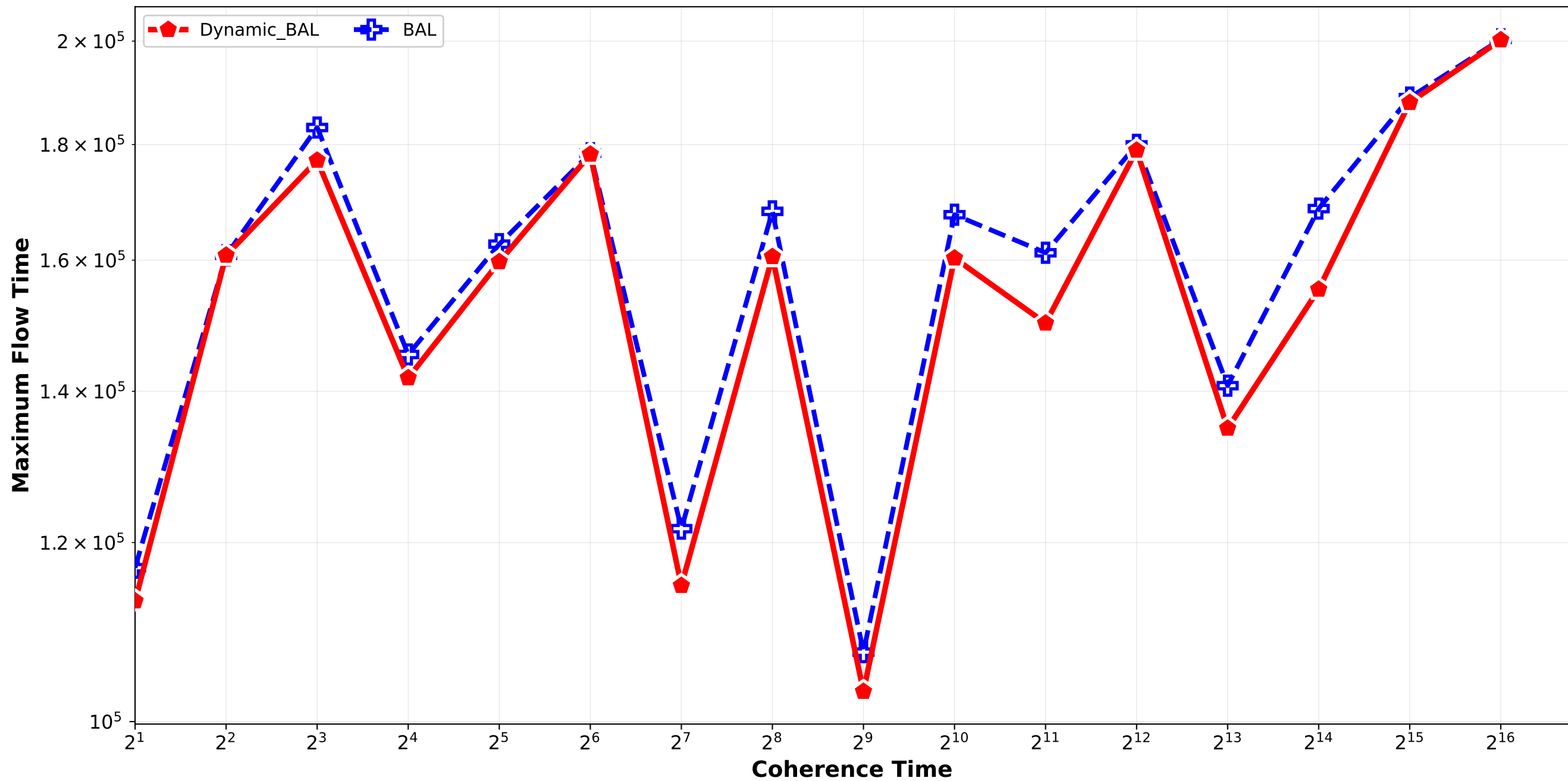
Dynamic_BAL vs BAL - Maximum Flow Time Bounded_Pareto_combination_random H512_H4096_H32768_H262144 / quadruplet_2
