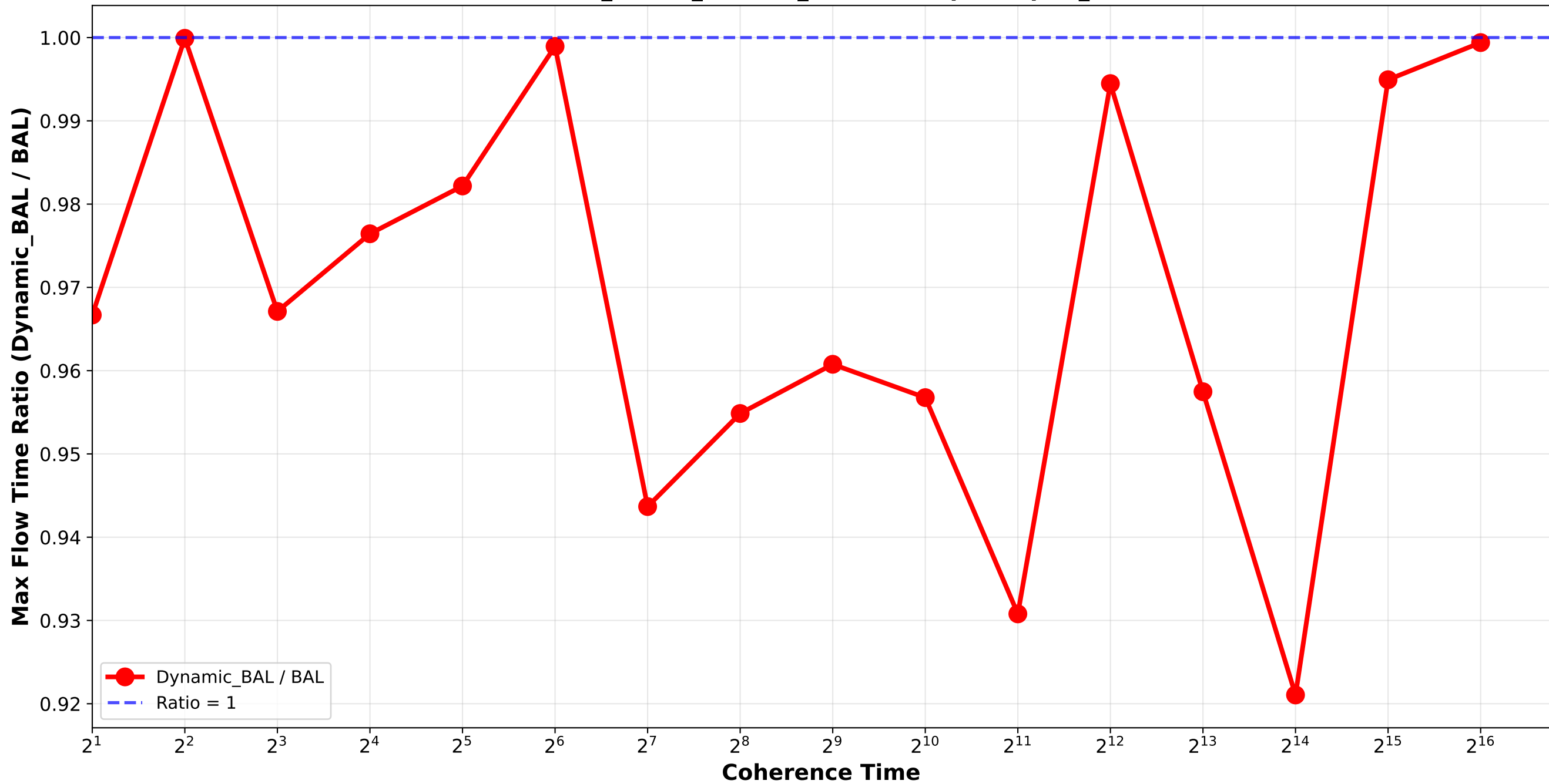
Dynamic_BAL vs BAL - Max Flow Time Ratio Bounded_Pareto_combination_random H512_H4096_H32768_H262144 / quadruplet_2
