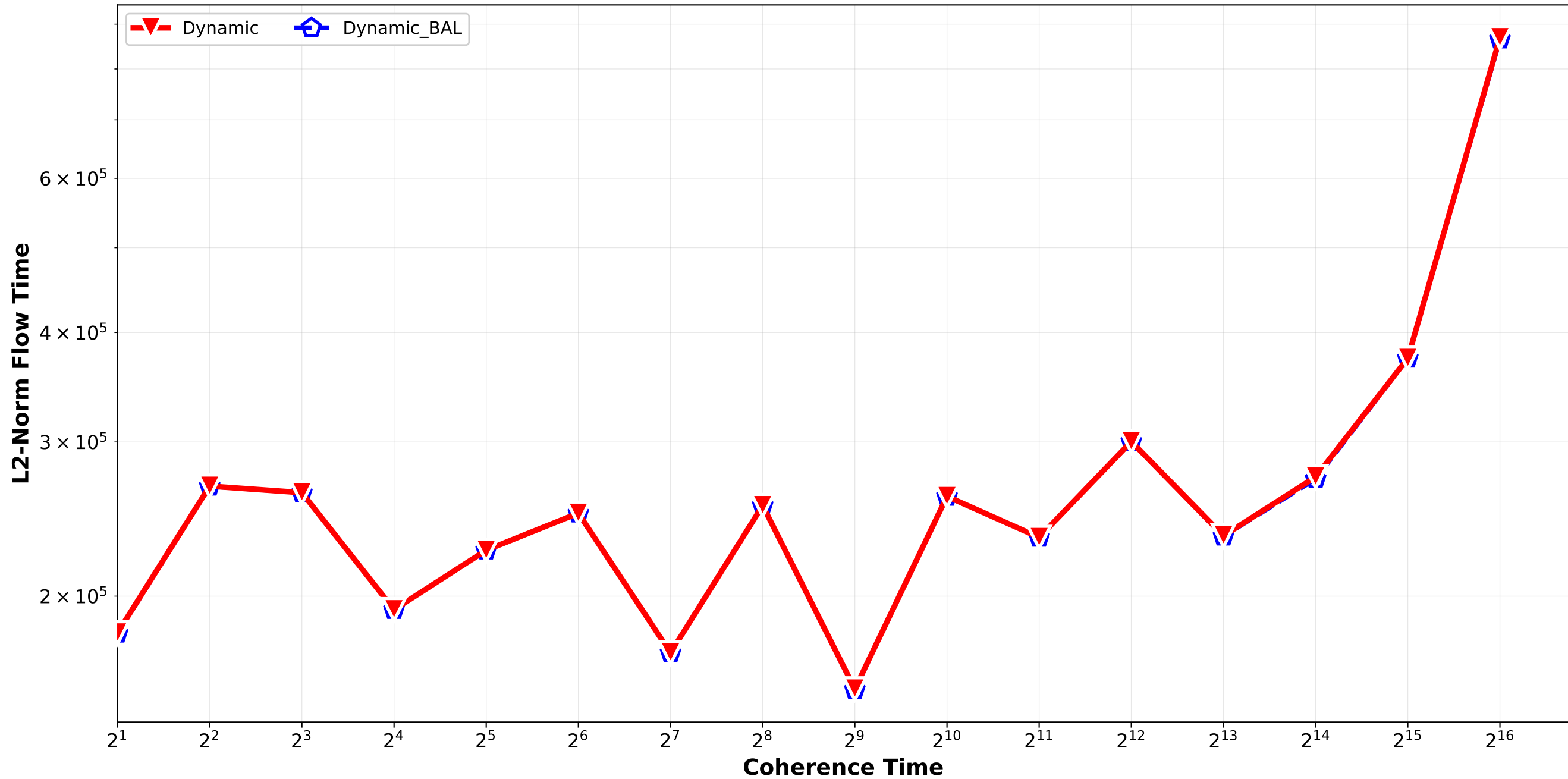
Dynamic vs Dynamic_BAL - L2 Norm Flow Time Bounded_Pareto_combination_random H512_H4096_H32768_H262144 / quadruplet_2
