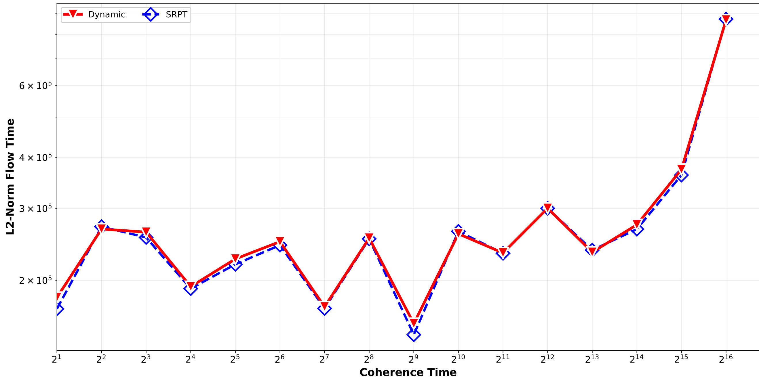
Dynamic vs SRPT - L2 Norm Flow Time Bounded_Pareto_combination_random H512_H4096_H32768_H262144 / quadruplet_2
