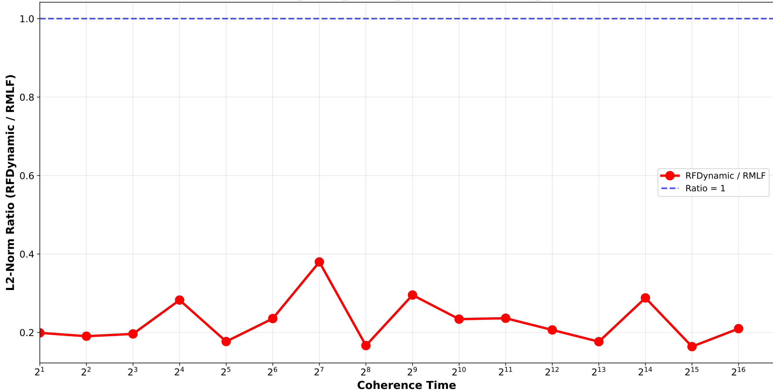
RFDynamic vs RMLF - L2 Norm Ratio Bounded_Pareto_combination_random H512_H4096_H32768_H262144 / quadruplet_2
