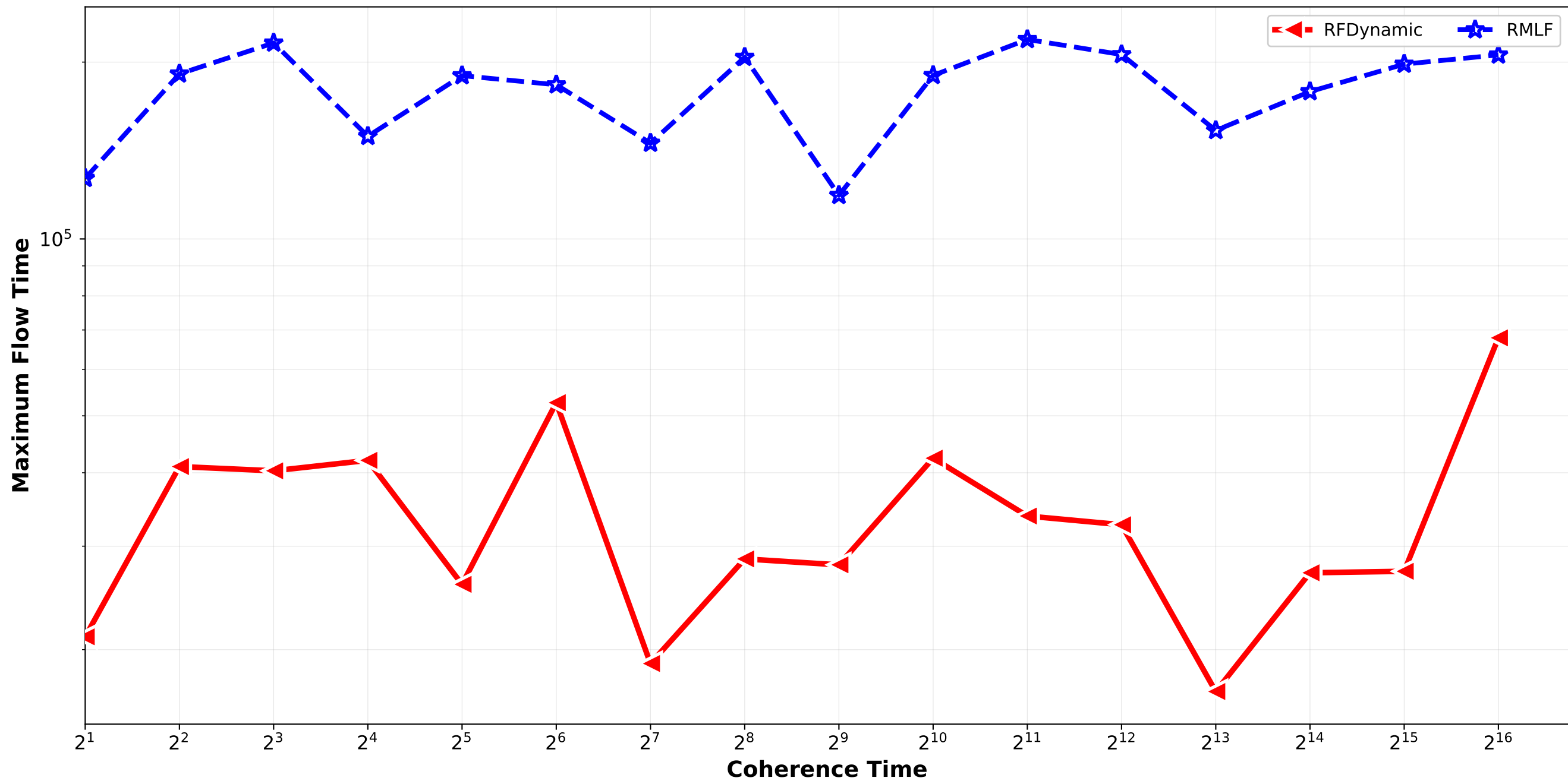
RFDynamic vs RMLF - Maximum Flow Time Bounded_Pareto_combination_random H512_H4096_H32768_H262144 / quadruplet_2
