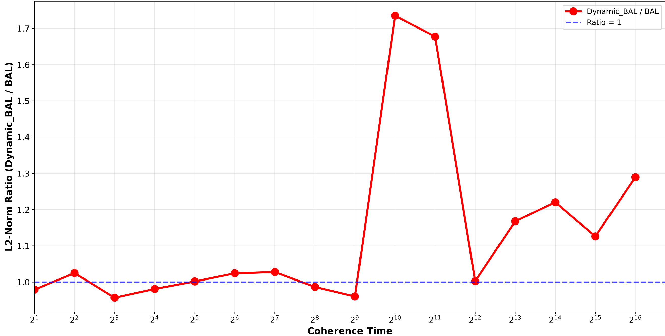
Dynamic_BAL vs BAL - L2 Norm Ratio Bounded_Pareto_combination_random H64_H512_H4096_H32768 / quadruplet_1
