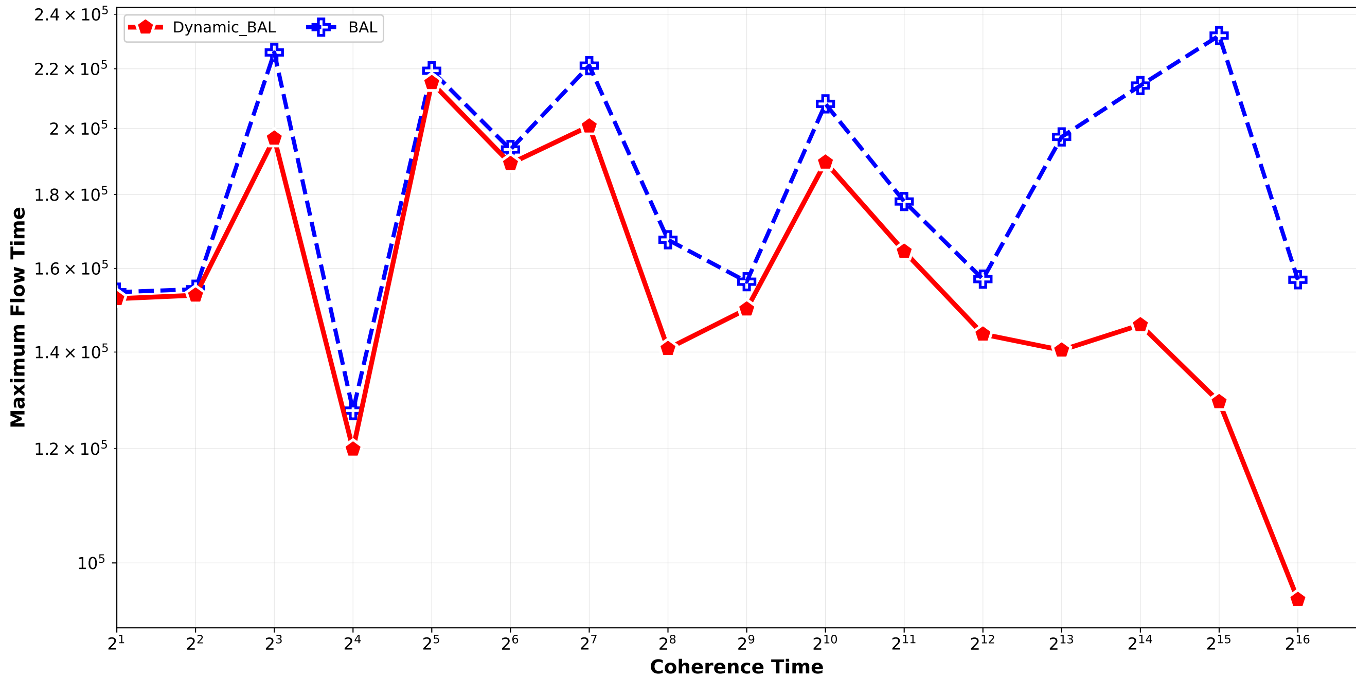
Dynamic_BAL vs BAL - Maximum Flow Time Bounded_Pareto_combination_random H64_H512_H4096_H32768 / quadruplet_1
