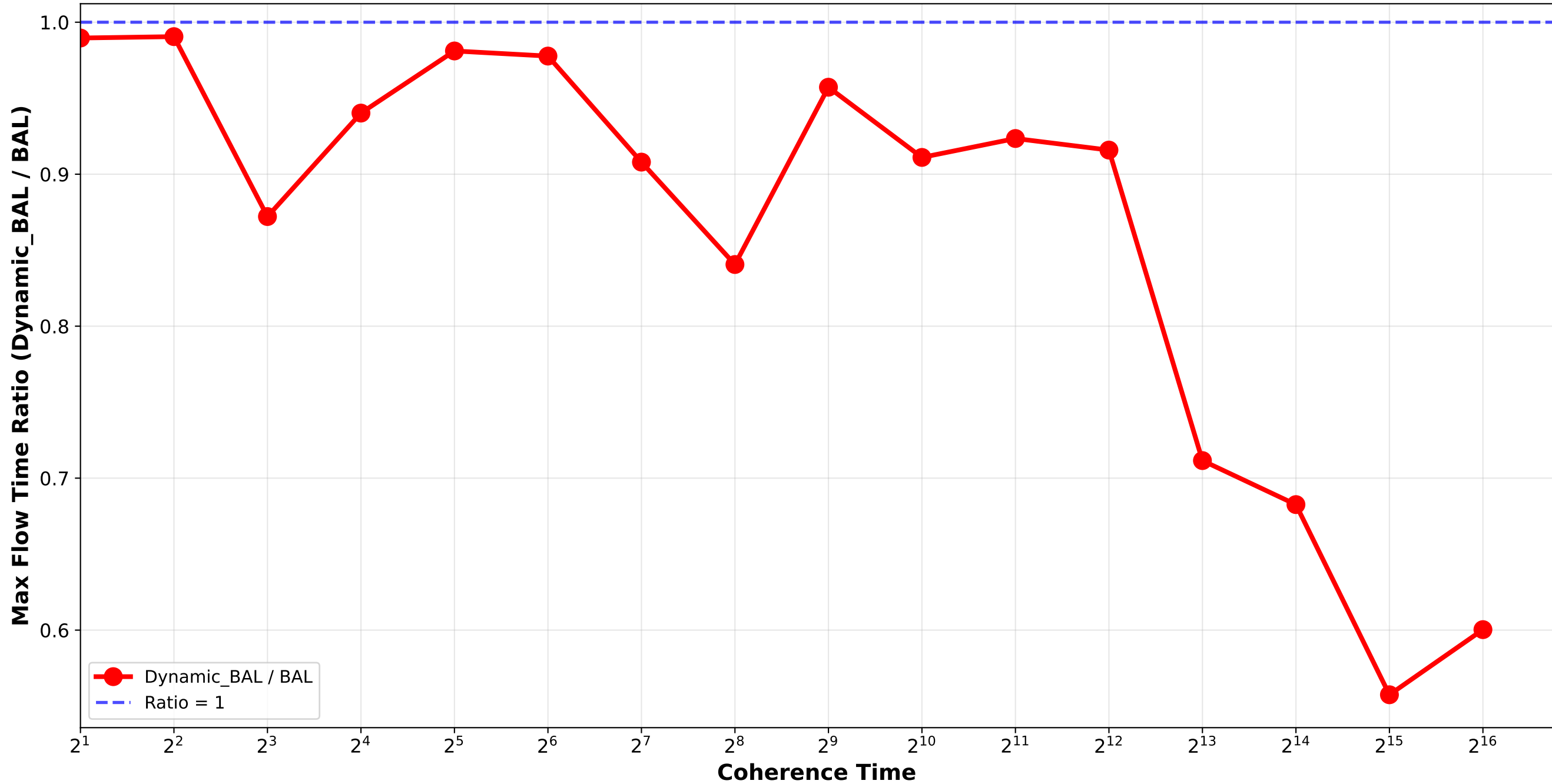
Dynamic_BAL vs BAL - Max Flow Time Ratio Bounded_Pareto_combination_random H64_H512_H4096_H32768 / quadruplet_1
