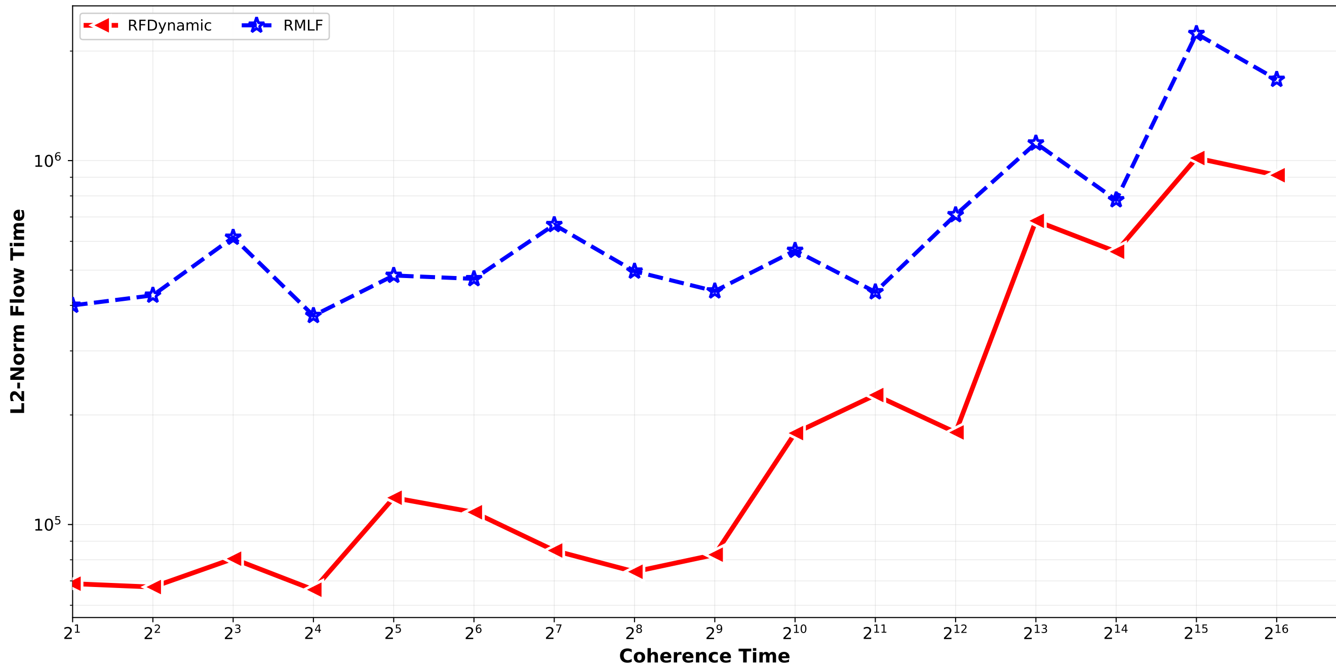
RFDynamic vs RMLF- L2 Norm Flow Time Bounded_Pareto_combination_random H64_H512_H4096_H32768 / quadruplet_1
