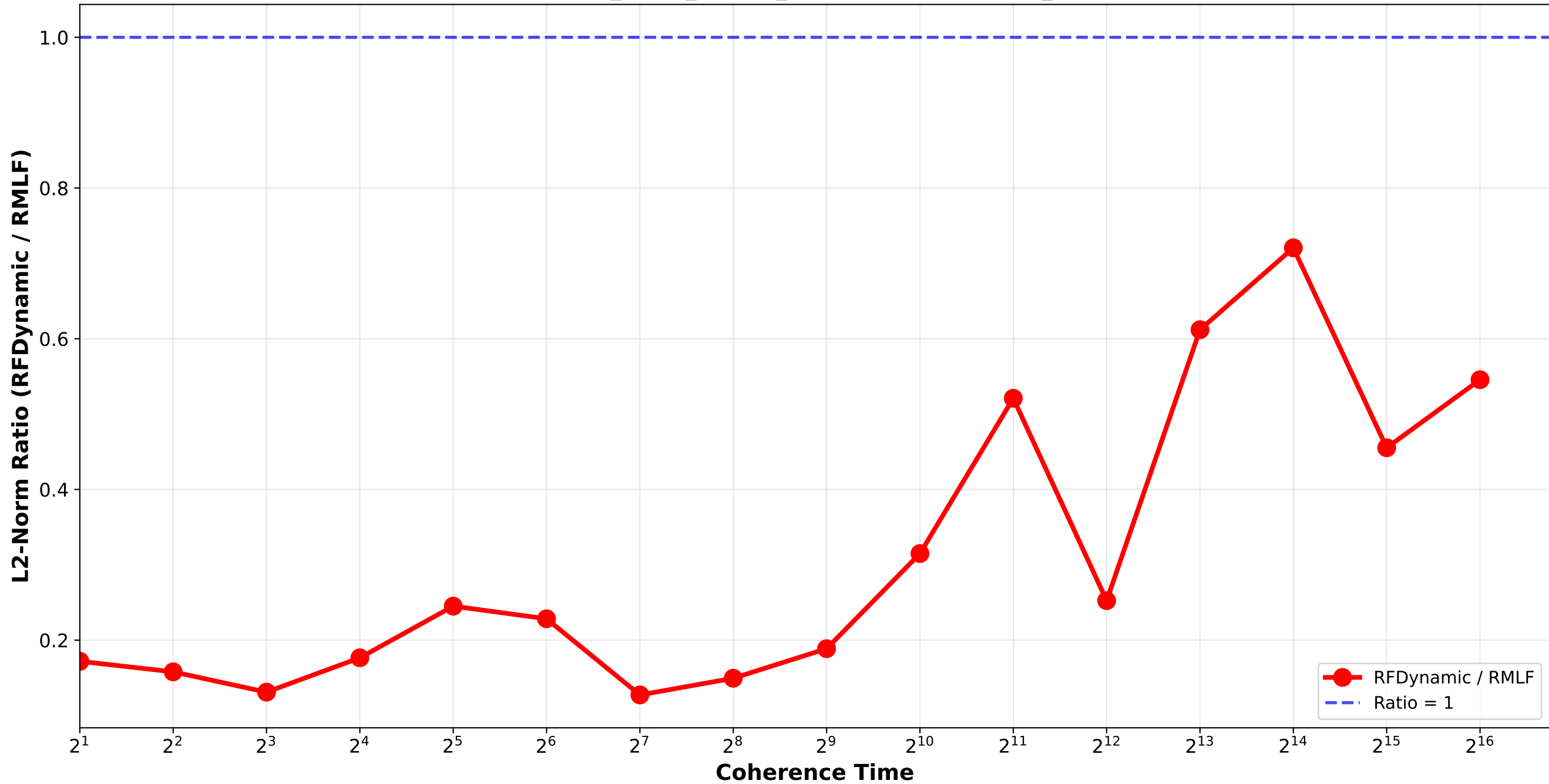
RFDynamic vs RMLF - L2 Norm Ratio Bounded_Pareto_combination_random H64_H512_H4096_H32768 / quadruplet_1
