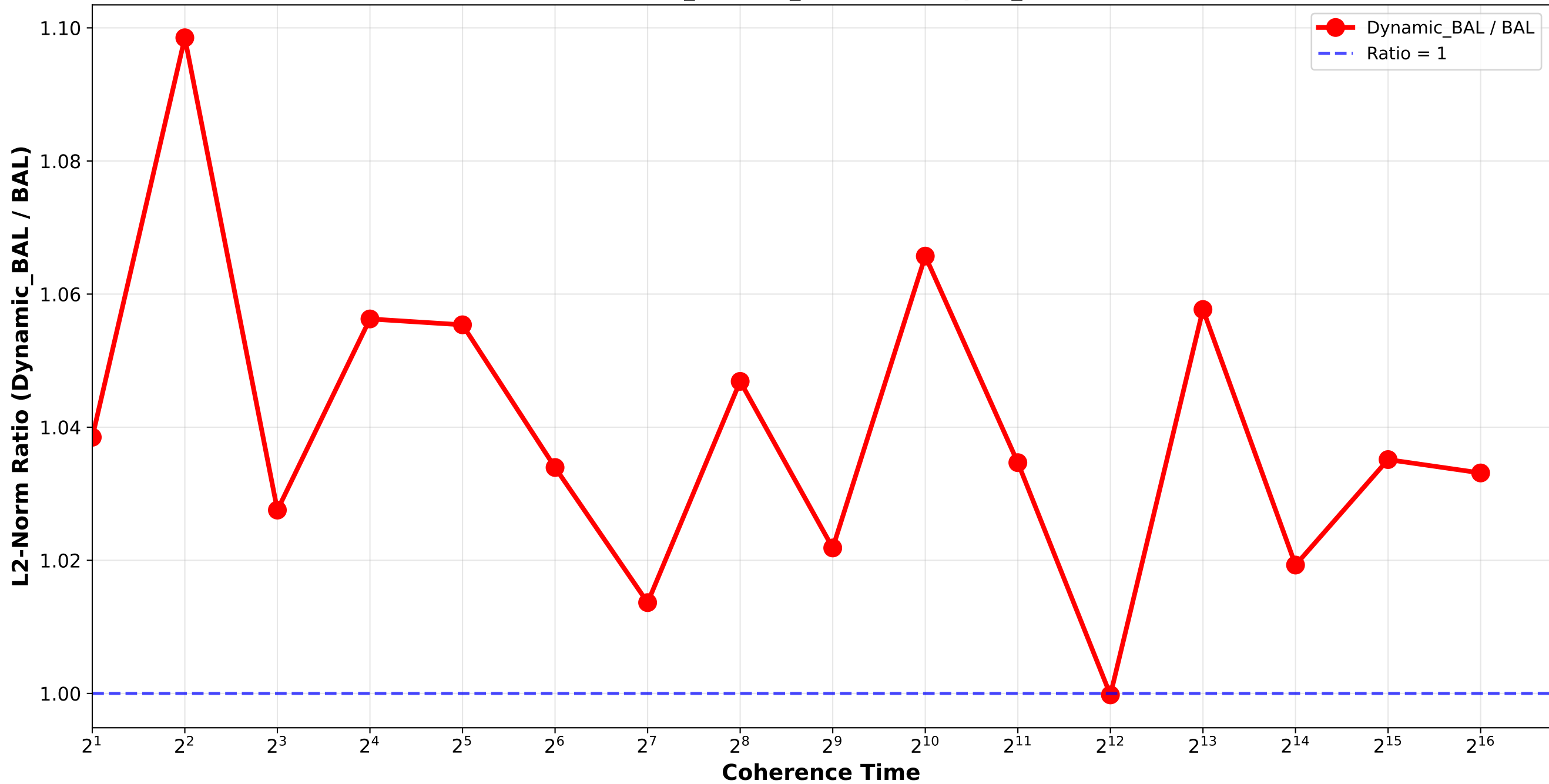
Dynamic_BAL vs BAL - L2 Norm Ratio Bounded_Pareto_combination_random H4096_H32768_H262144 / triplet_3
