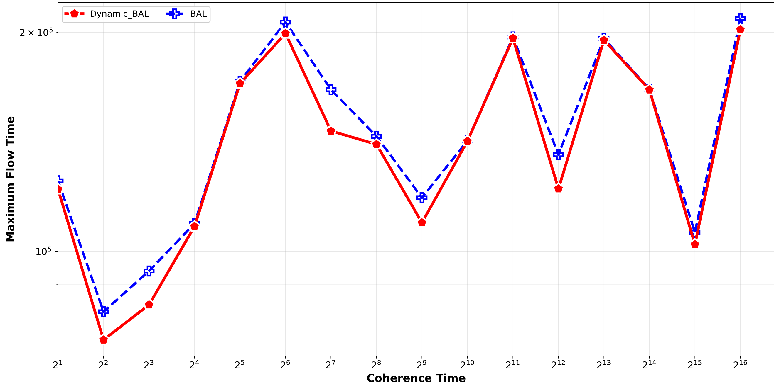
Dynamic_BAL vs BAL - Maximum Flow Time Bounded_Pareto_combination_random H4096_H32768_H262144 / triplet_3
