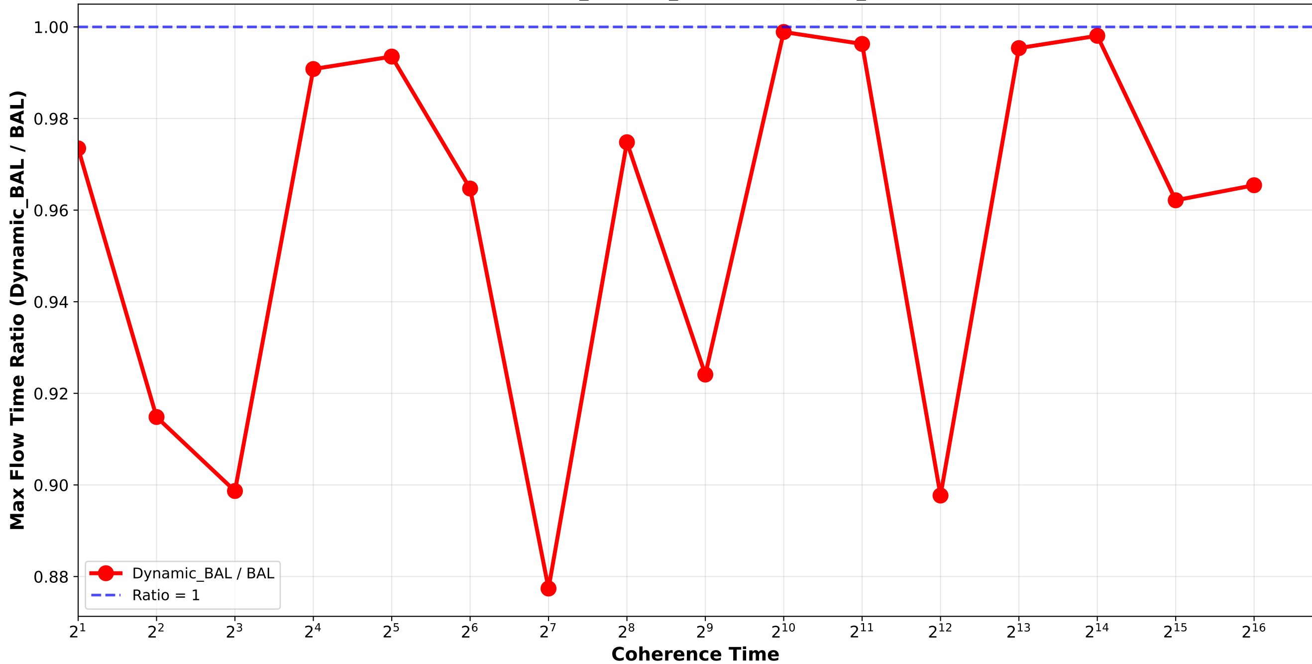
Dynamic_BAL vs BAL - Max Flow Time Ratio Bounded_Pareto_combination_random H4096_H32768_H262144 / triplet_3
