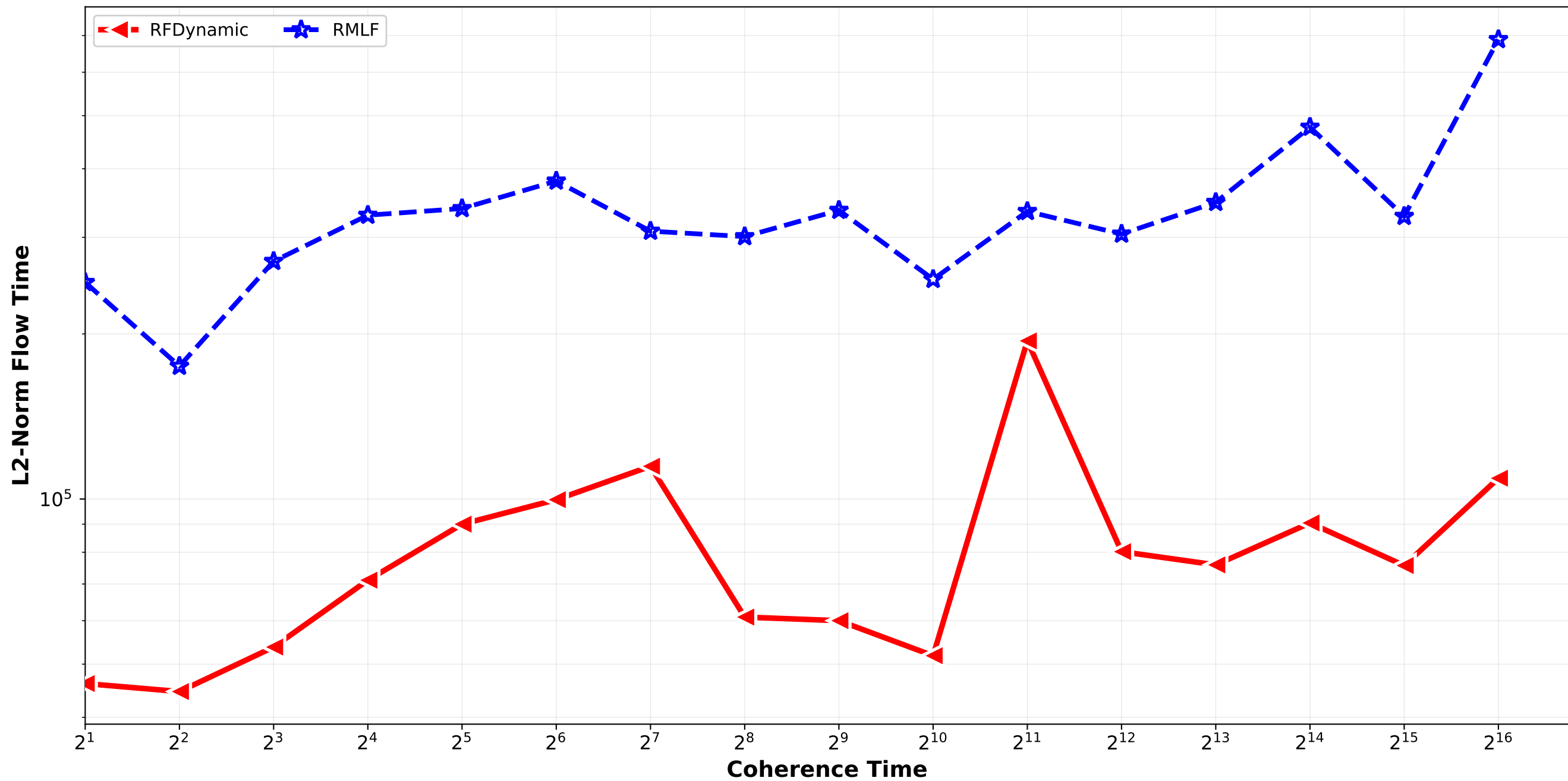
RFDynamic vs RMLF- L2 Norm Flow Time Bounded_Pareto_combination_random H4096_H32768_H262144 / triplet_3
