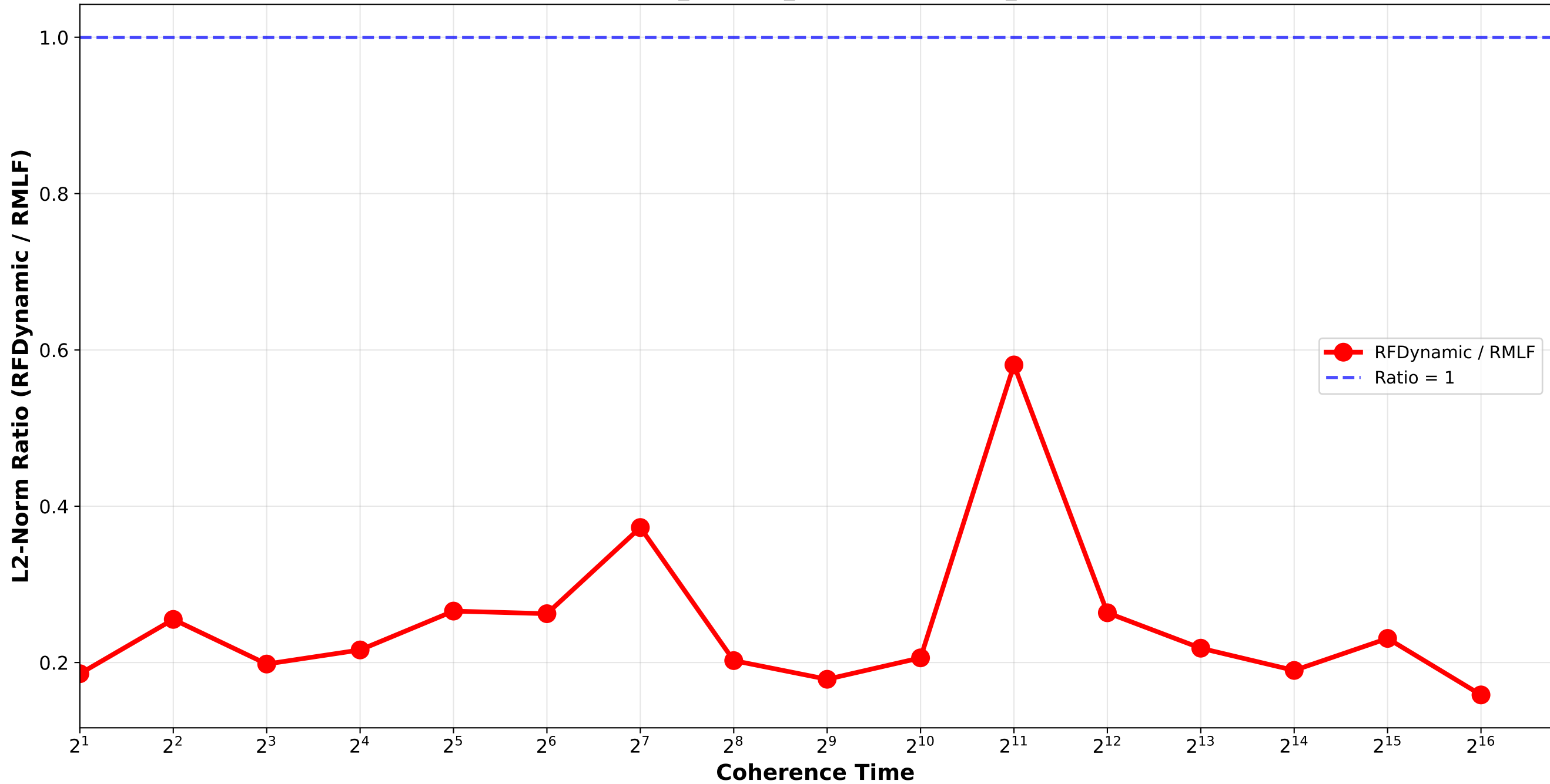
RFDynamic vs RMLF - L2 Norm Ratio Bounded_Pareto_combination_random H4096_H32768_H262144 / triplet_3
