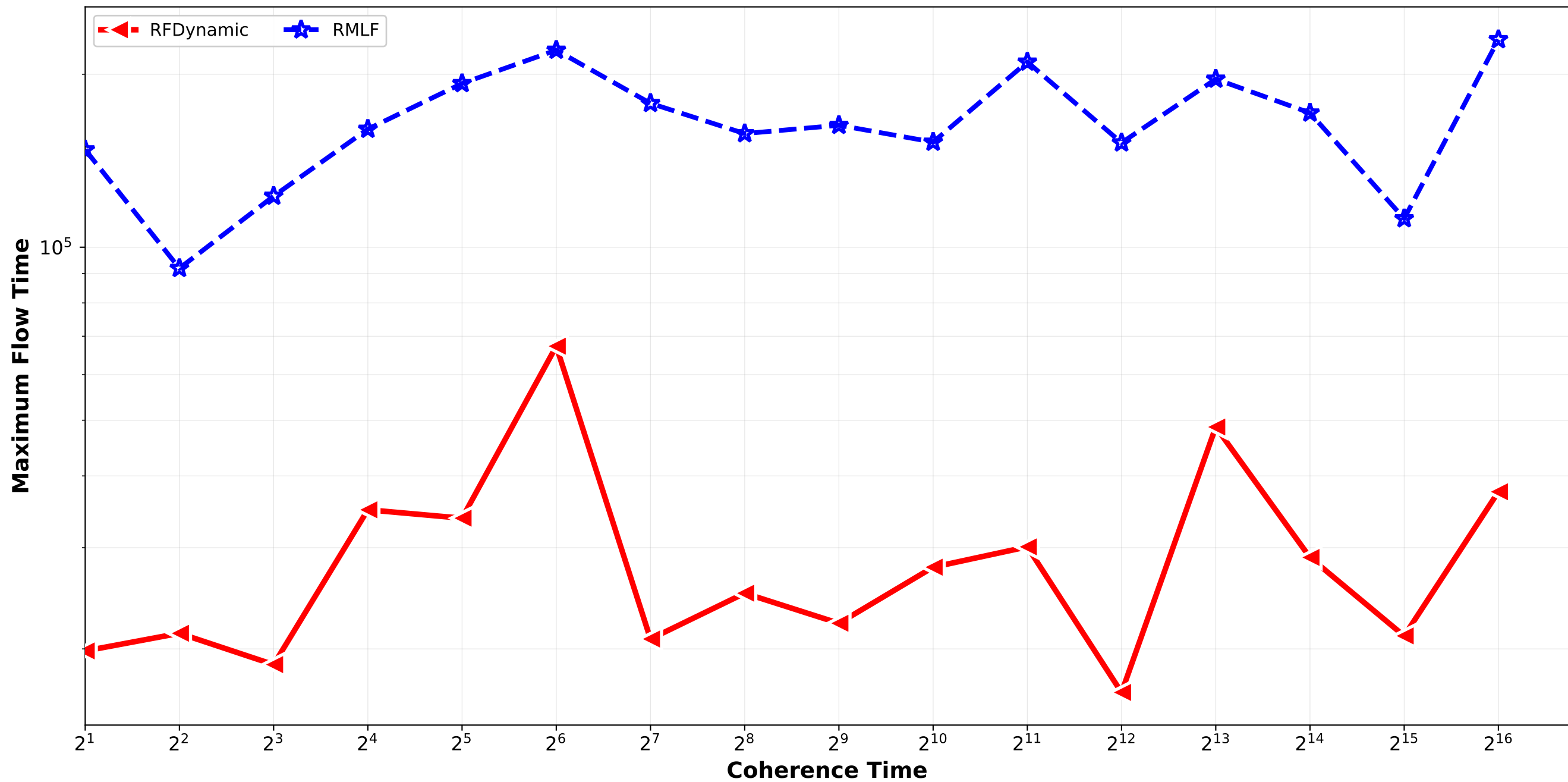
RFDynamic vs RMLF - Maximum Flow Time Bounded_Pareto_combination_random H4096_H32768_H262144 / triplet_3
