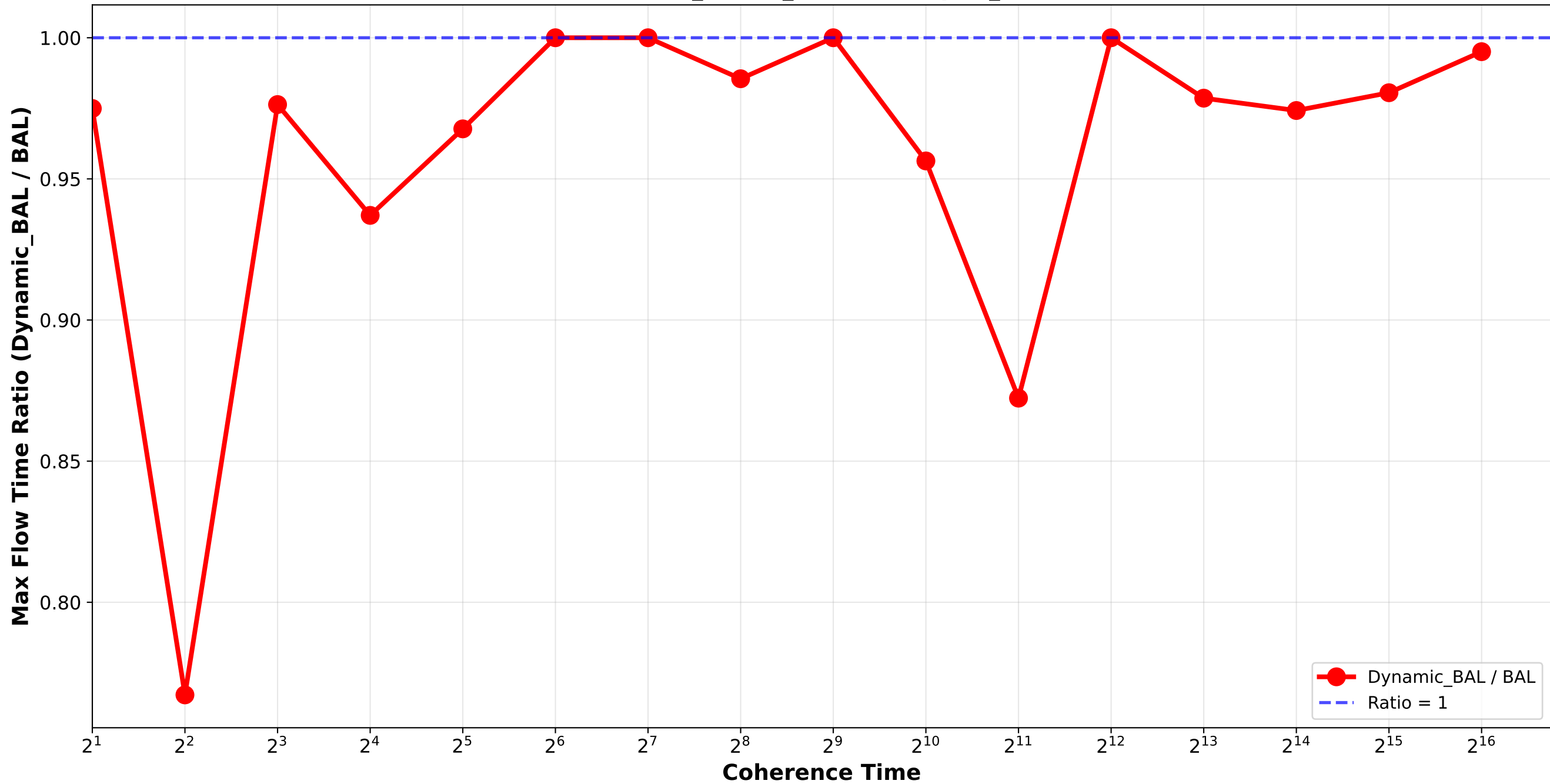
Dynamic_BAL vs BAL - Max Flow Time Ratio Bounded_Pareto_combination_random H512_H4096_H32768 / triplet_2
