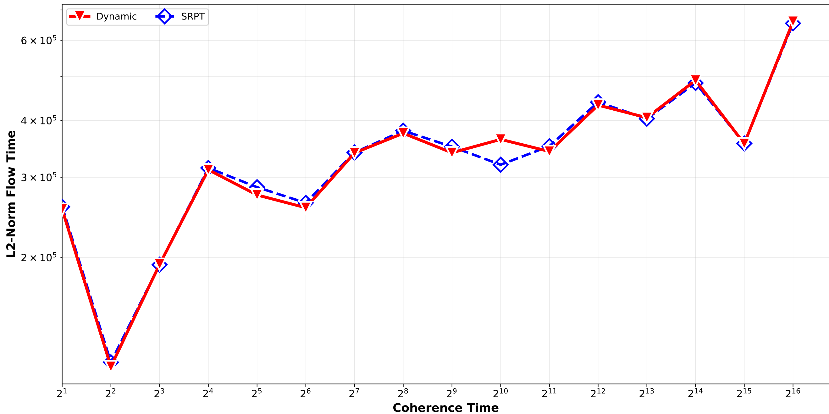
Dynamic vs SRPT - L2 Norm Flow Time Bounded_Pareto_combination_random H512_H4096_H32768 / triplet_2
