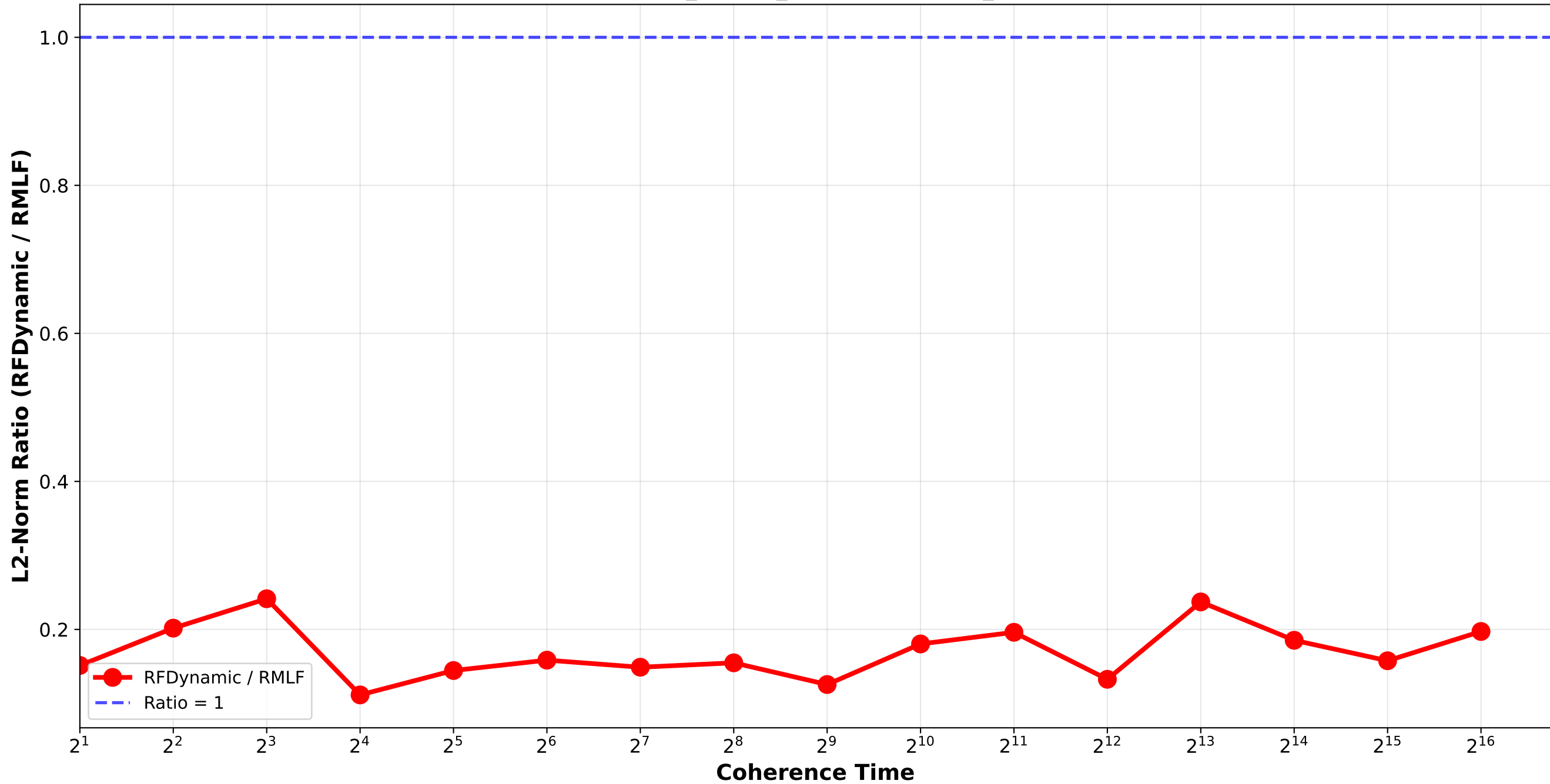
RFDynamic vs RMLF - L2 Norm Ratio Bounded_Pareto_combination_random H512_H4096_H32768 / triplet_2
