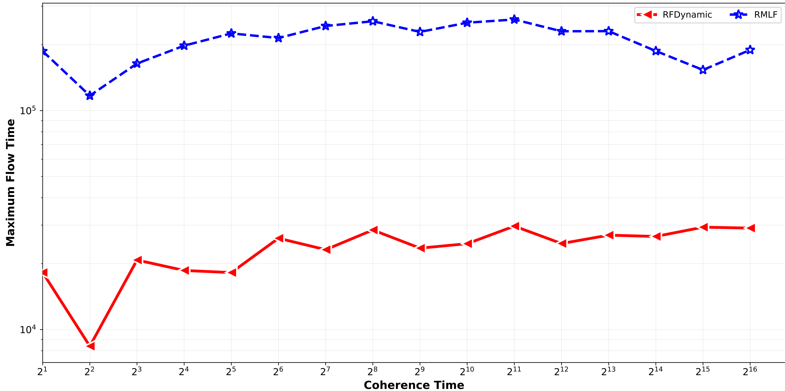
RFDynamic vs RMLF - Maximum Flow Time Bounded_Pareto_combination_random H512_H4096_H32768 / triplet_2
