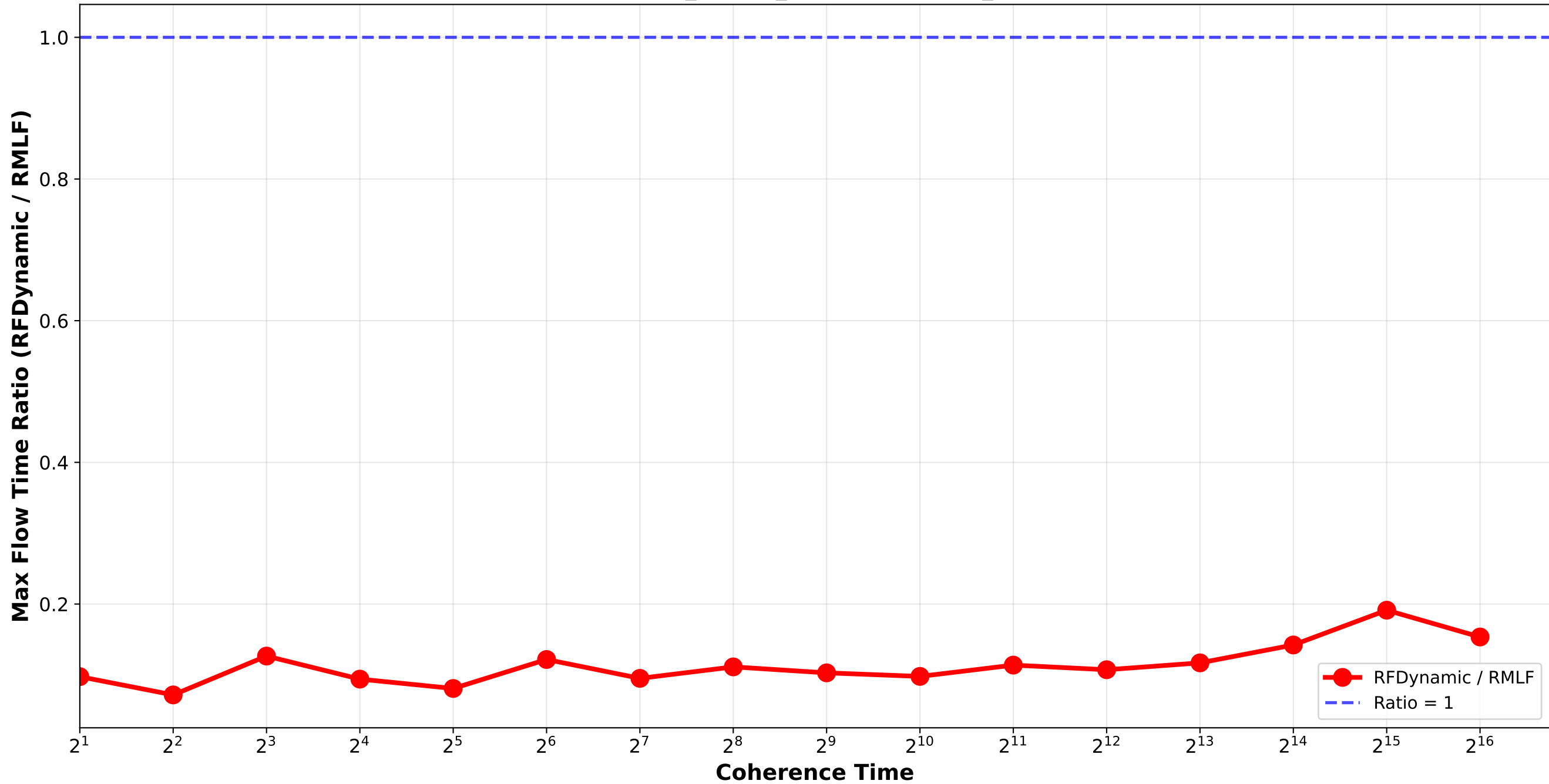
RFDynamic vs RMLF - Max Flow Time Ratio Bounded_Pareto_combination_random H512_H4096_H32768 / triplet_2
