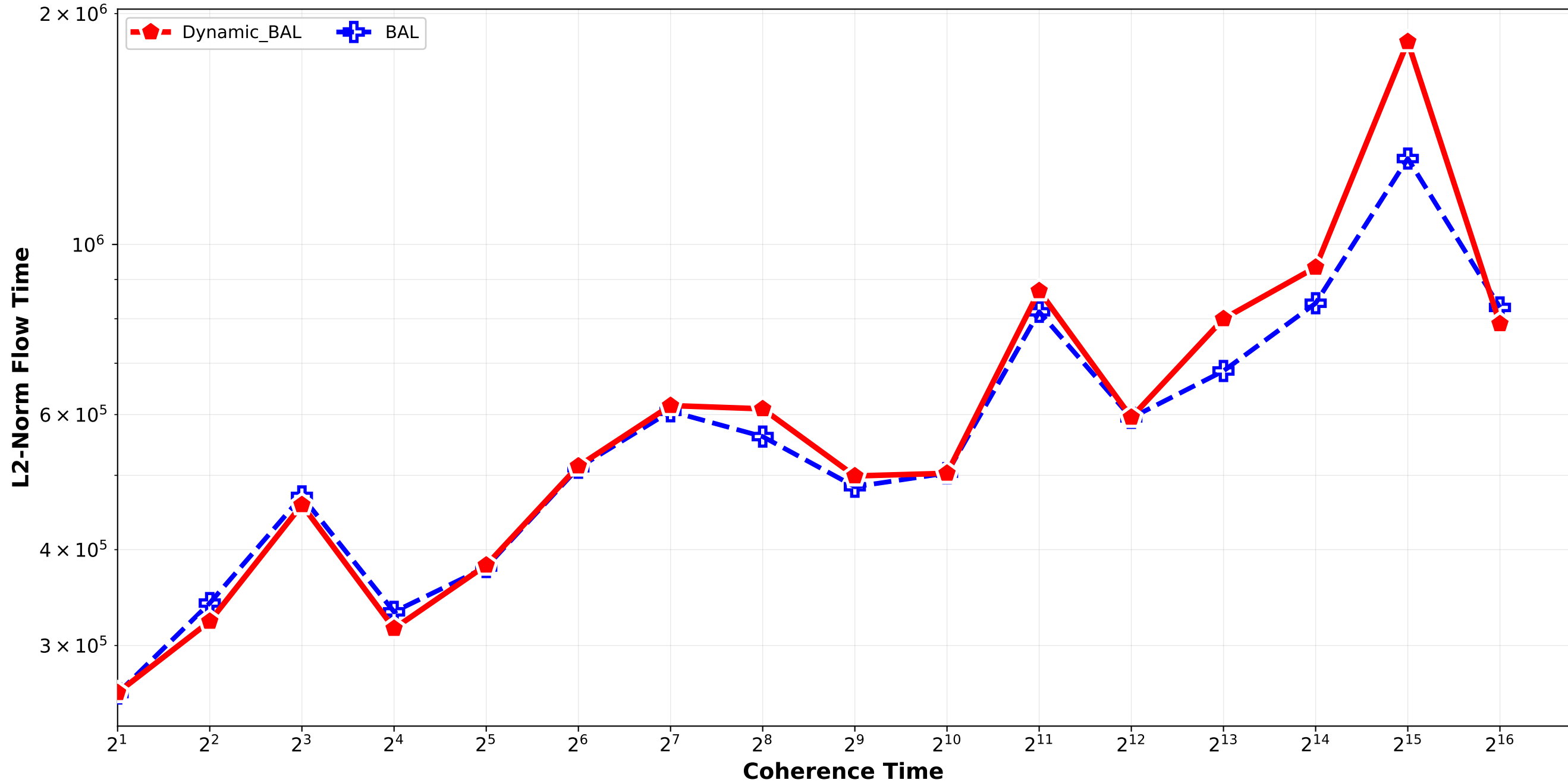
Dynamic_BAL vs BAL - L2 Norm Flow Time Bounded_Pareto_combination_random H64_H512_H4096 / triplet_1
