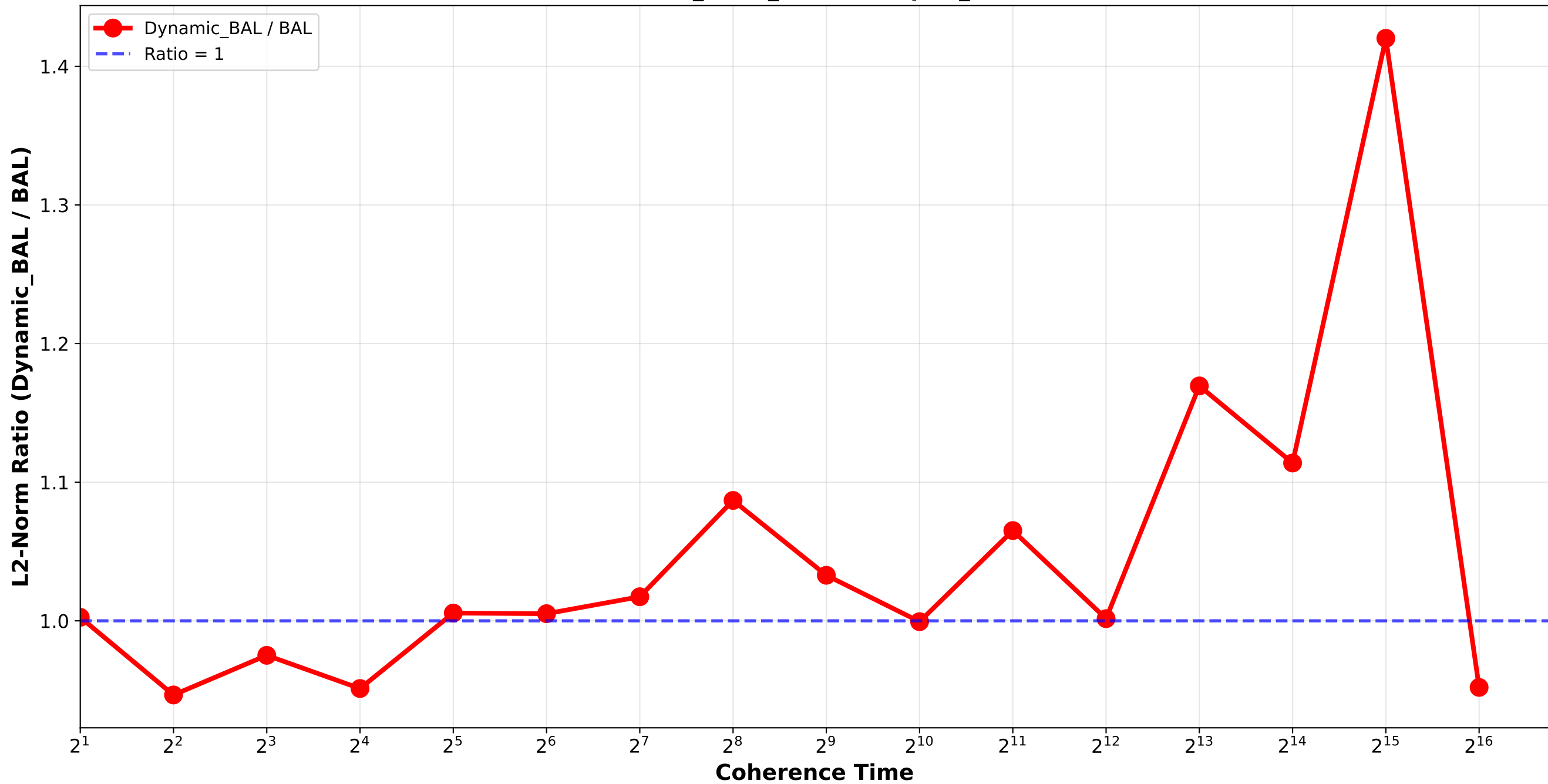
Dynamic_BAL vs BAL - L2 Norm Ratio Bounded_Pareto_combination_random H64_H512_H4096 / triplet_1
